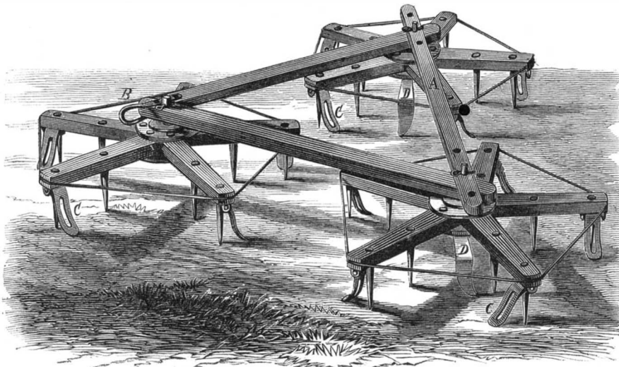
BATES' PATENT REVOLVING AUTOMATIC HARROW.
