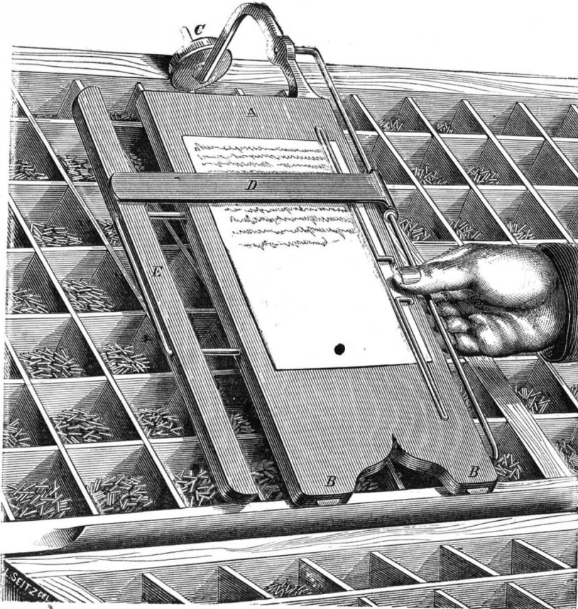
LA FRANCE'S PATENT COPY HOLDER AND GUIDE.
