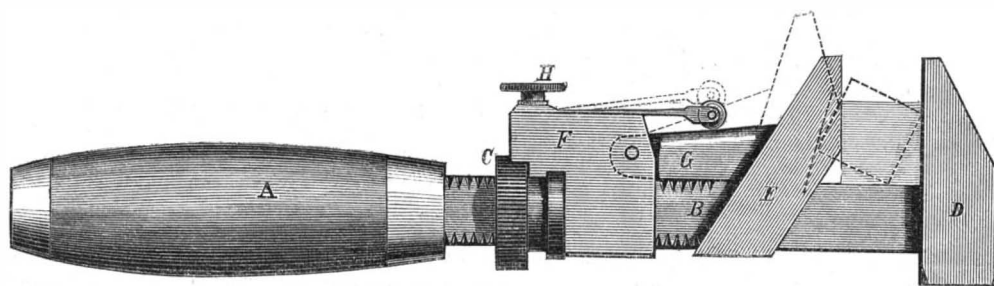
BRADSHAW & LYON'S SPRING-JAW WRENCH.
