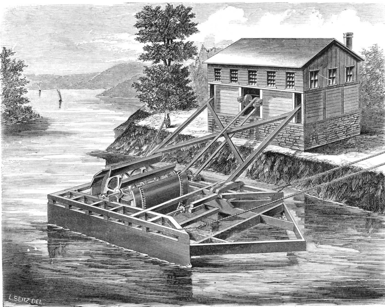
SHEPARD'S PATENT CURRENT MILL.
