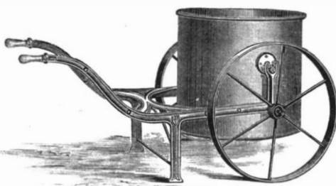
Fig. 20. - Waite, Burnell & Co.'s Swinging Tub Barrow. Capacities 82 to 225 liters. Price 75 to 180 francs.
