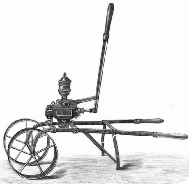
Fig. 21. - Beame's Pump Barrow. Horizontal Action. Capacity 2,500 liters per hour. Complete with Suction and Discharge Pipes, etc. 126 francs. Capacity 5,000 to 6,000 liters per hour, 215 francs.
