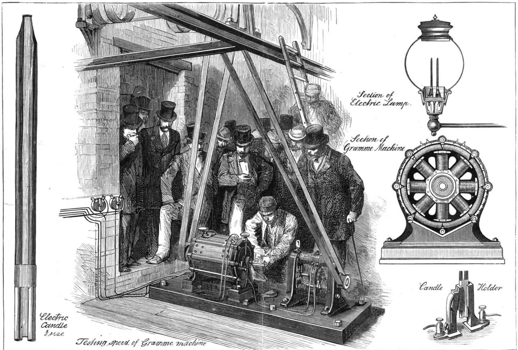
THE ELECTRIC LIGHT.—SKETCH OF THE APPARATUS.
