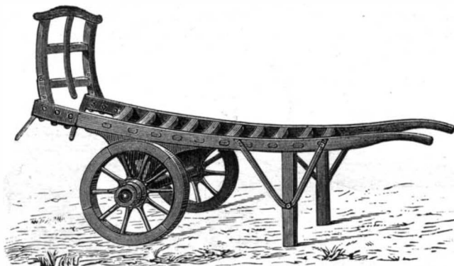
Fig. 5.—Wheelbarrow for Railway Stations.—(Model of Orleans.)
