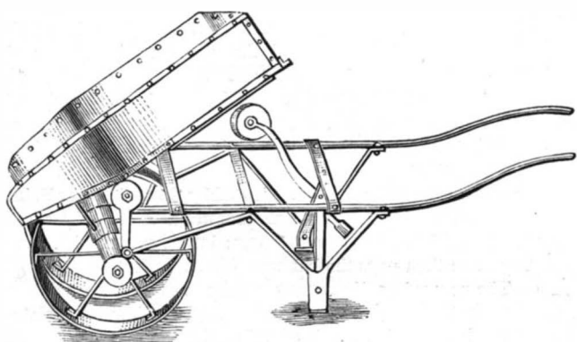
Fig. 9.—Dumping Barrow.
