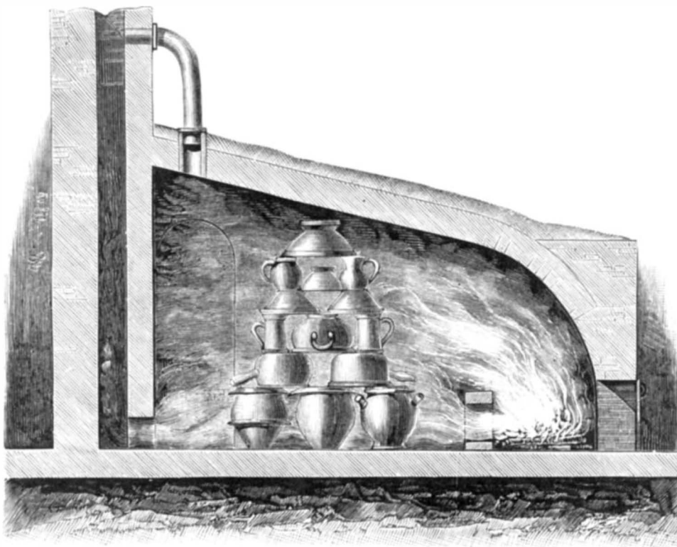
Fig. 1.—POTTER'S OVEN.
