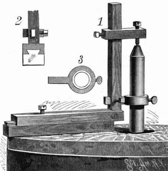
DAVIS' MILLSTONE PAINT STAFF.
