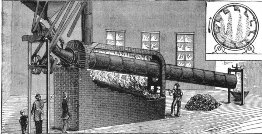
WORRELL'S COMBINED DRIER AND COOLER.
