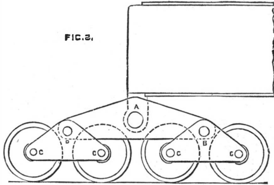
FIG. 2. ONE CORNER OF THE CARRIAGE.
