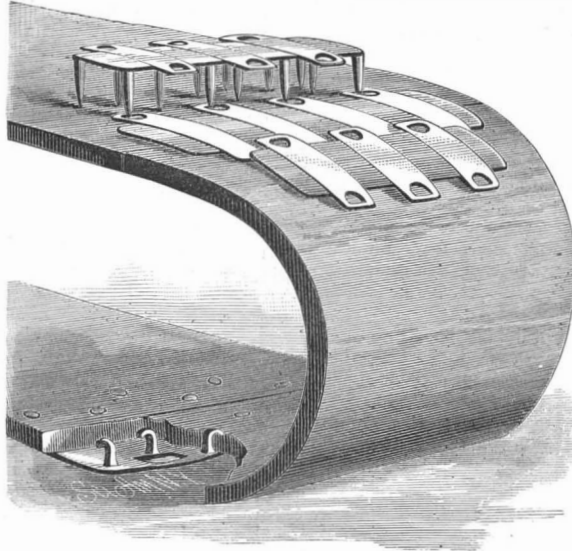
NEW BELT FASTENER.
