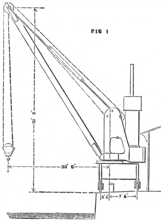
FIG. 1. OUTLINE OF THE CRANE.
