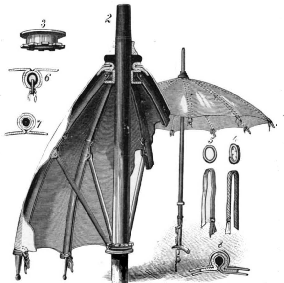
LOCKLING'S IMPROVED UMBRELLA.
