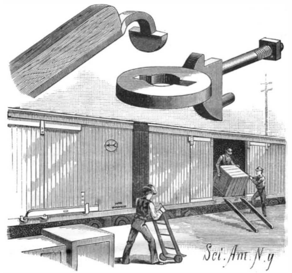
ROWE'S FREIGHT CAR SKID.
