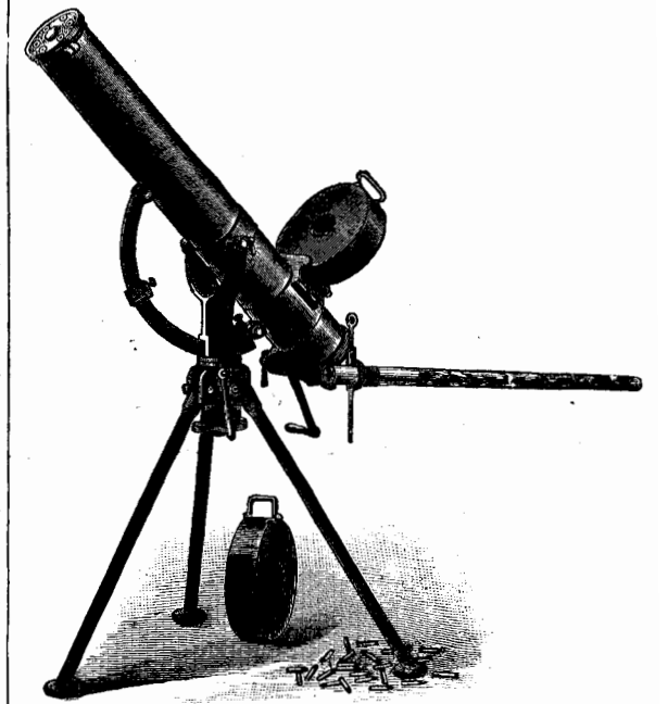
Fig. 4.—GATLING GUN MOUNTED ON TRIPOD.
