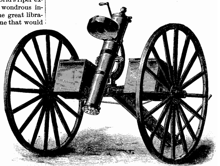
Fig. 2.—SHOWING DEPRESSION AT WHICH GATLING GUN CAN BE FIRED.
