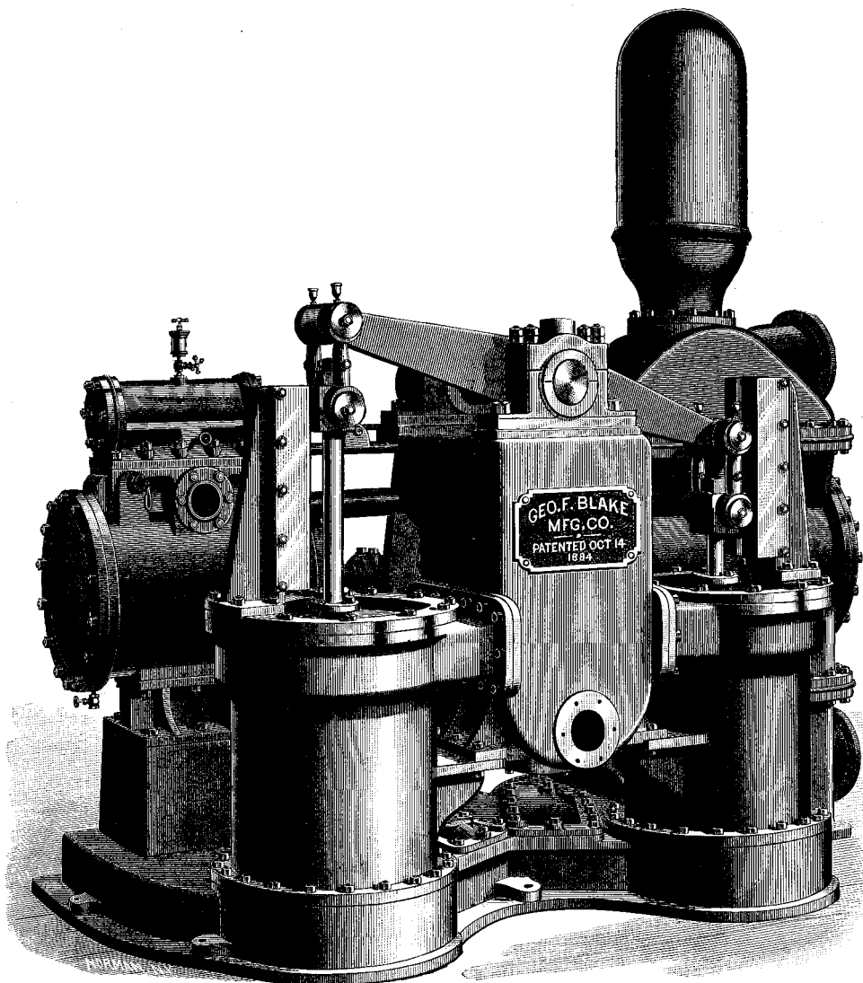
PUMPING ENGINES FOR U. S. CRUISER CHICAGO.
