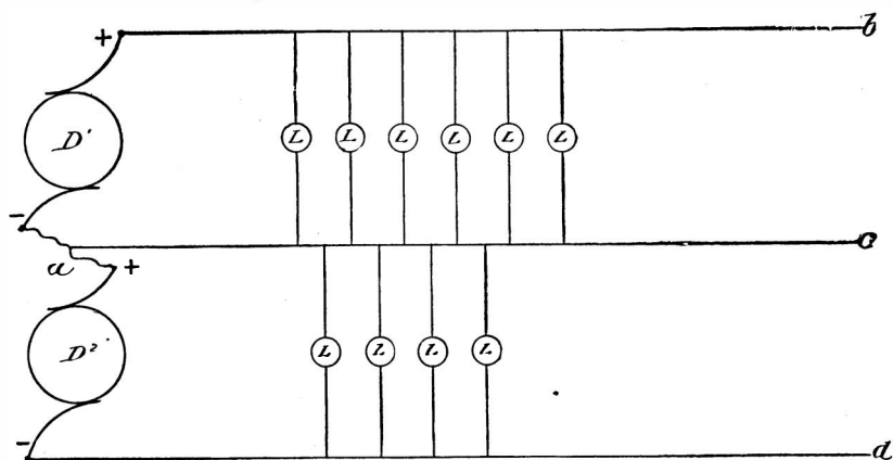
Fig. 4.—EDISON THREE-WIRE SYSTEM.
