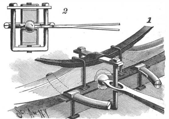
LOWE'S VEHICLE RUNNING GEAR.
