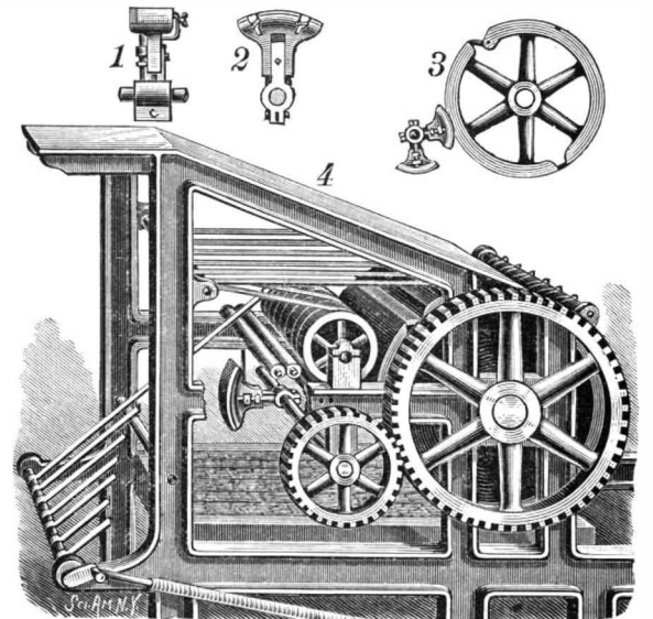
DITSON'S PRINTING PRESS ATTACHMENT.
