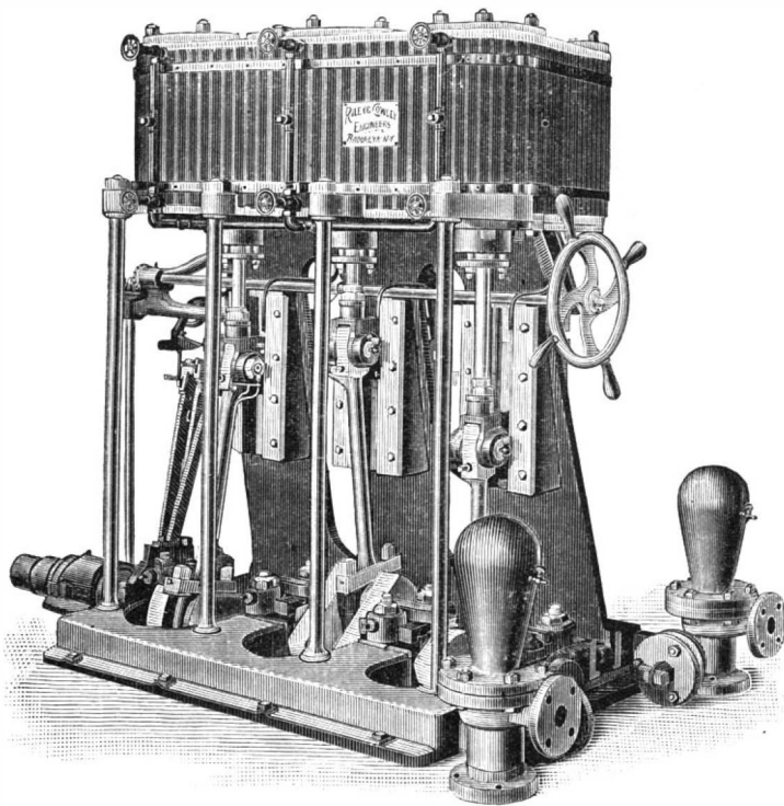
TRIPLE EXPANSION ENGINE FOR STEEL LAUNCH "LILLIAN."
