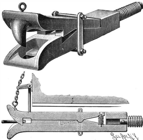
MONROE & YEAGER'S CAR COUPLING. #1.
