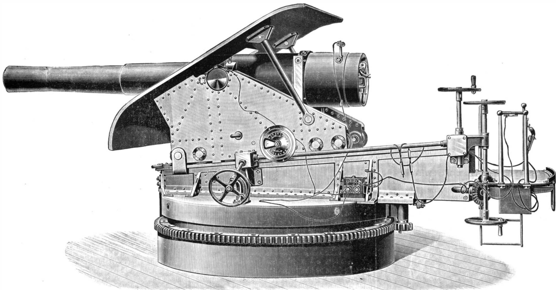
ARMSTRONG 92 INCH GUN MOUNTED.
