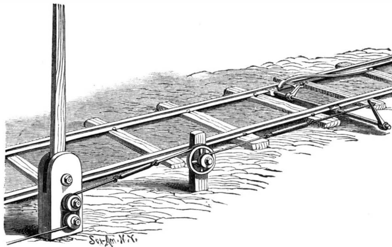
ANTHONY'S AUTOMATIC GATE FOR RAILWAY CROSSINGS.
