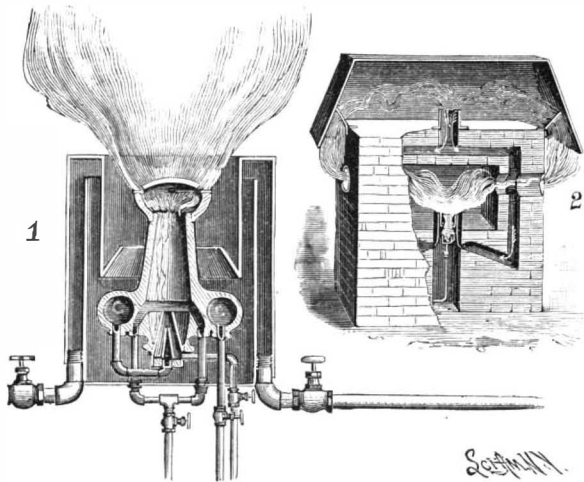
ANDREWS & SEERY'S HYDROCARBON BURNER.
