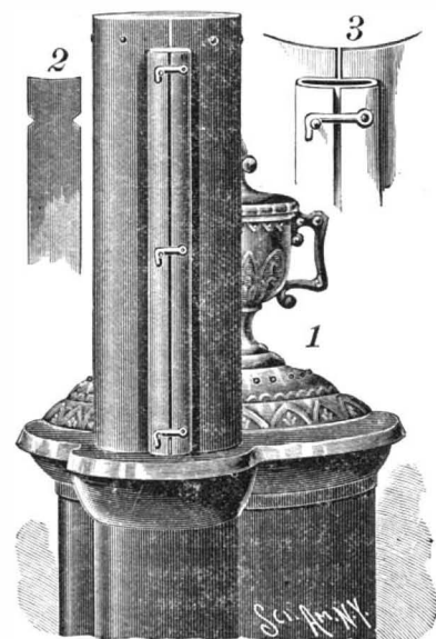
TURNER'S IMPROVED STOVE PIPE.
