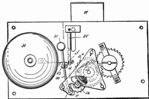
Fig. 2.—DE BASTO'S ALARM LOCK.
