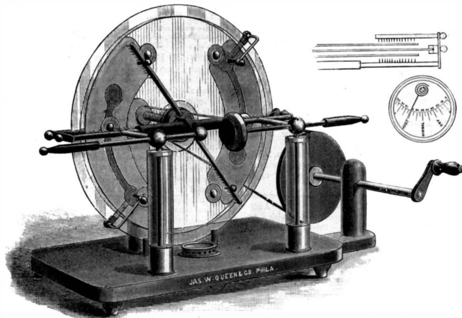
QUEEN'S NEW TRIPLE PLATE TOEPLER-HOLTZ MACHINE.
