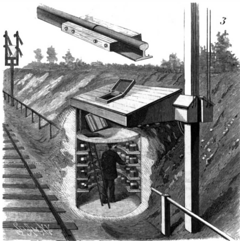
3. RELAY POLE AND BATTERY. 4. INSULATION OF RAIL ENDS.
