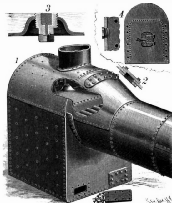
CRONIN'S IMPROVEMENTS IN STEAM BOILERS.
