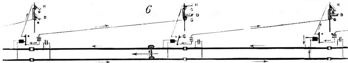
SINGLE SIGNAL BLOCKING.
