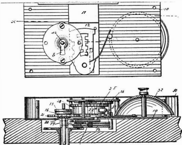
Fig. 1.—DE BASTO'S ALARM LOCK.
