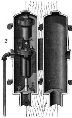
MECHANISM FOR MOVING SEMAPHORE, ETC.
