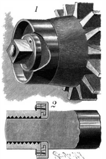
SULLIVAN'S NUT AND WASHER FOR VEHICLE AXLES.
