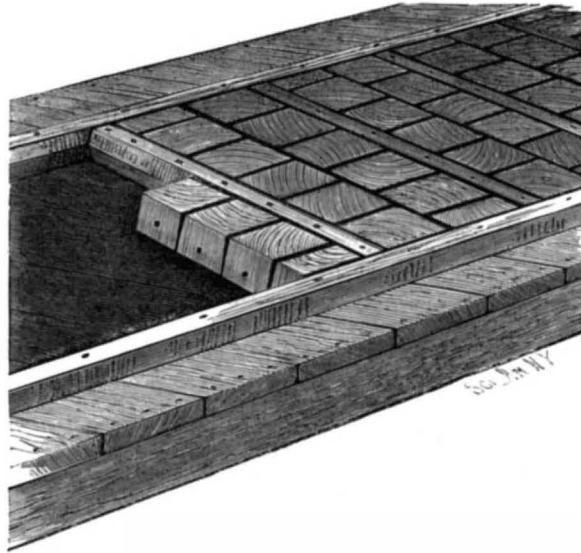
CARMAN'S BRIDGE FLOORING.
