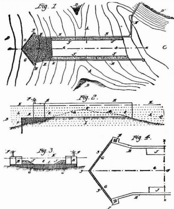
MAUERMANN'S PROTECTOR FOR SUBMARINE CHANNELS.
