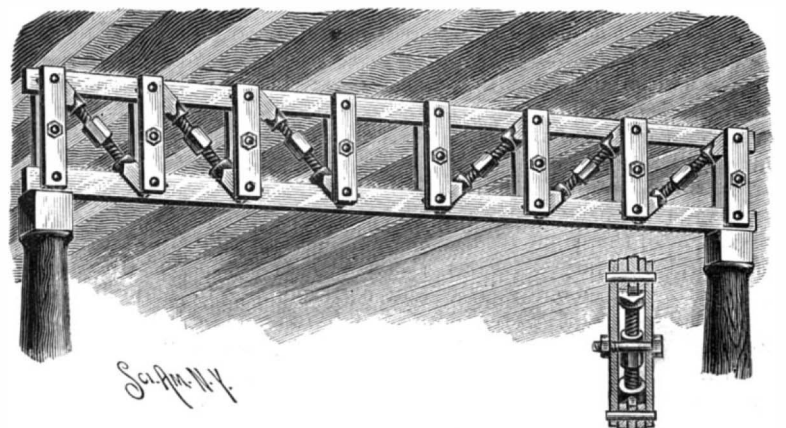
OLSEN'S LIFTING TRUSS GIRDER.
