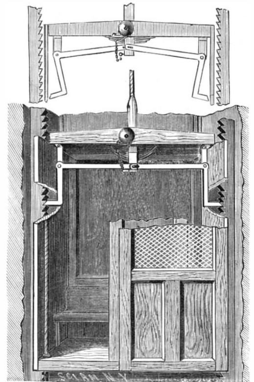
LYNN'S SAFETY INDICATOR FOR ELEVATORS.
