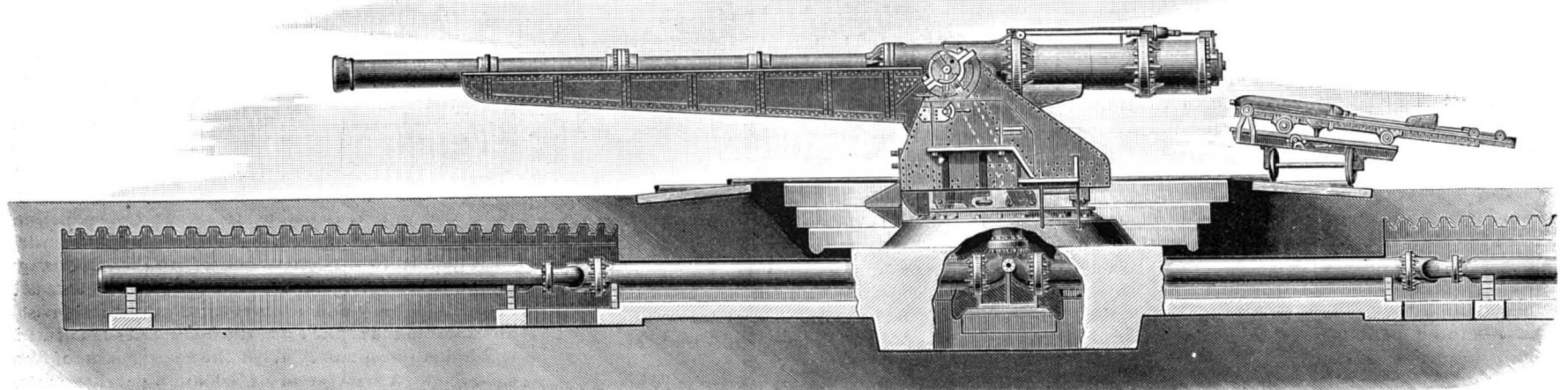
DYNAMITE GUN, SIDE ELEVATION, SHOWING LOADING CARRIAGE.
