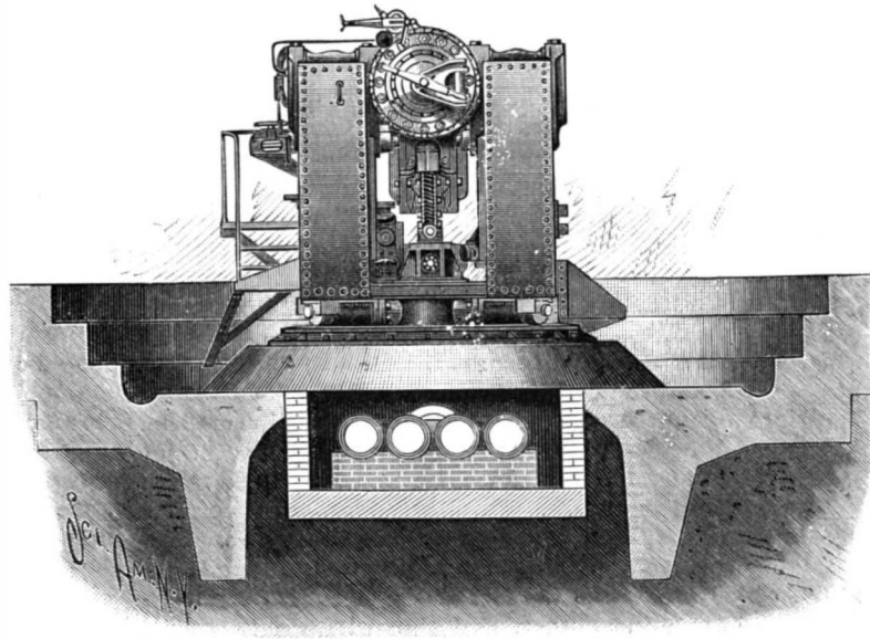
DYNAMITE GUN, END ELEVATION, PARTLY IN SECTION.
