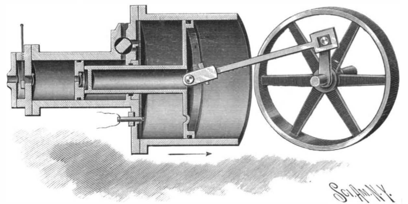
PARKER'S IMPROVED GAS ENGINE.
