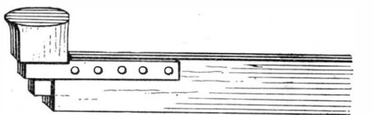
STEEL HEAD FOR SMOOTHING DOME.
