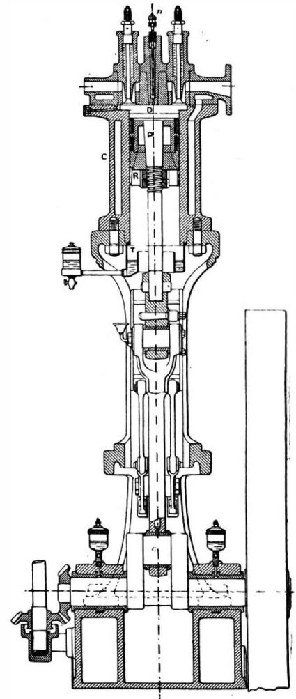
Fig. 3.—LONGITUDINAL SECTION.
