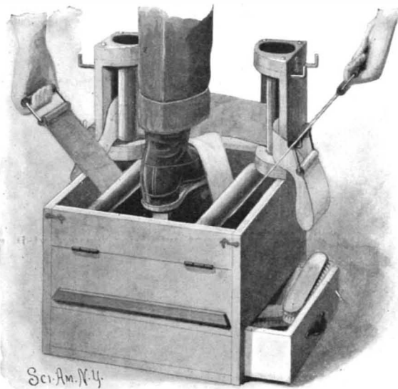
BURWELL'S POLISHING APPARATUS.
