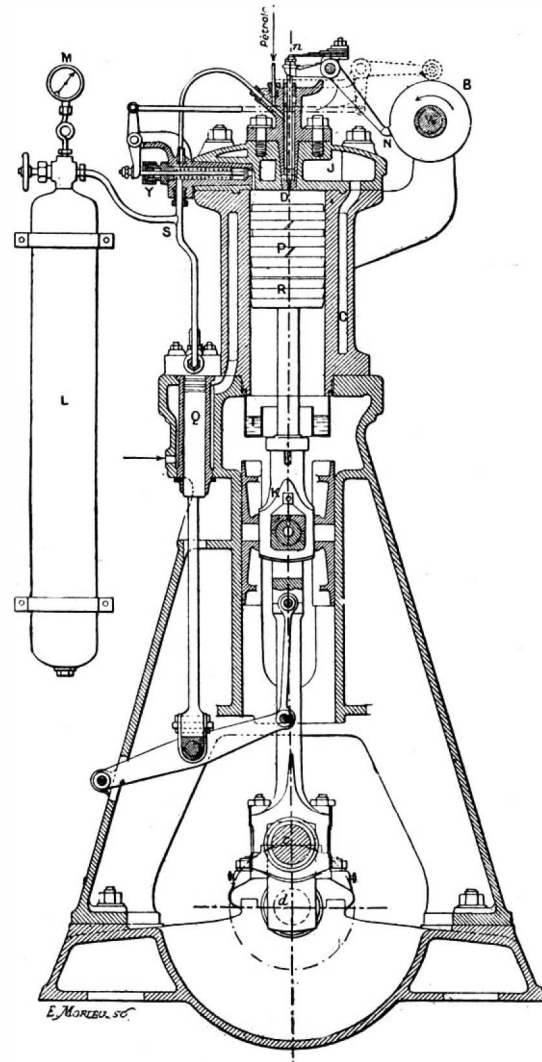
Fig. 2.—TRANSVERSE SECTION.
