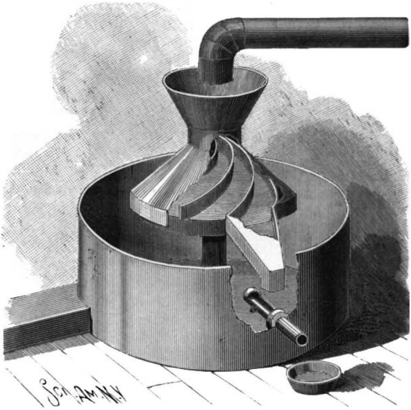
BYRNES' SAMPLING MACHINE.
