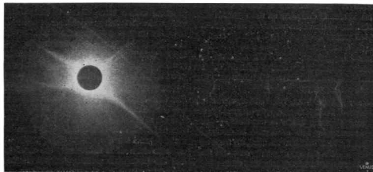
PHOTO OF SOLAR CORONA,
