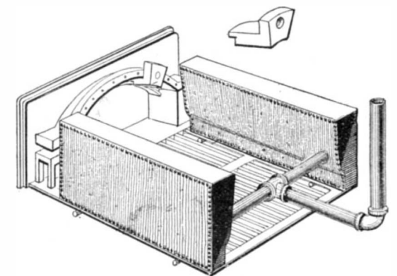
THE SKELETON-FRAME.
