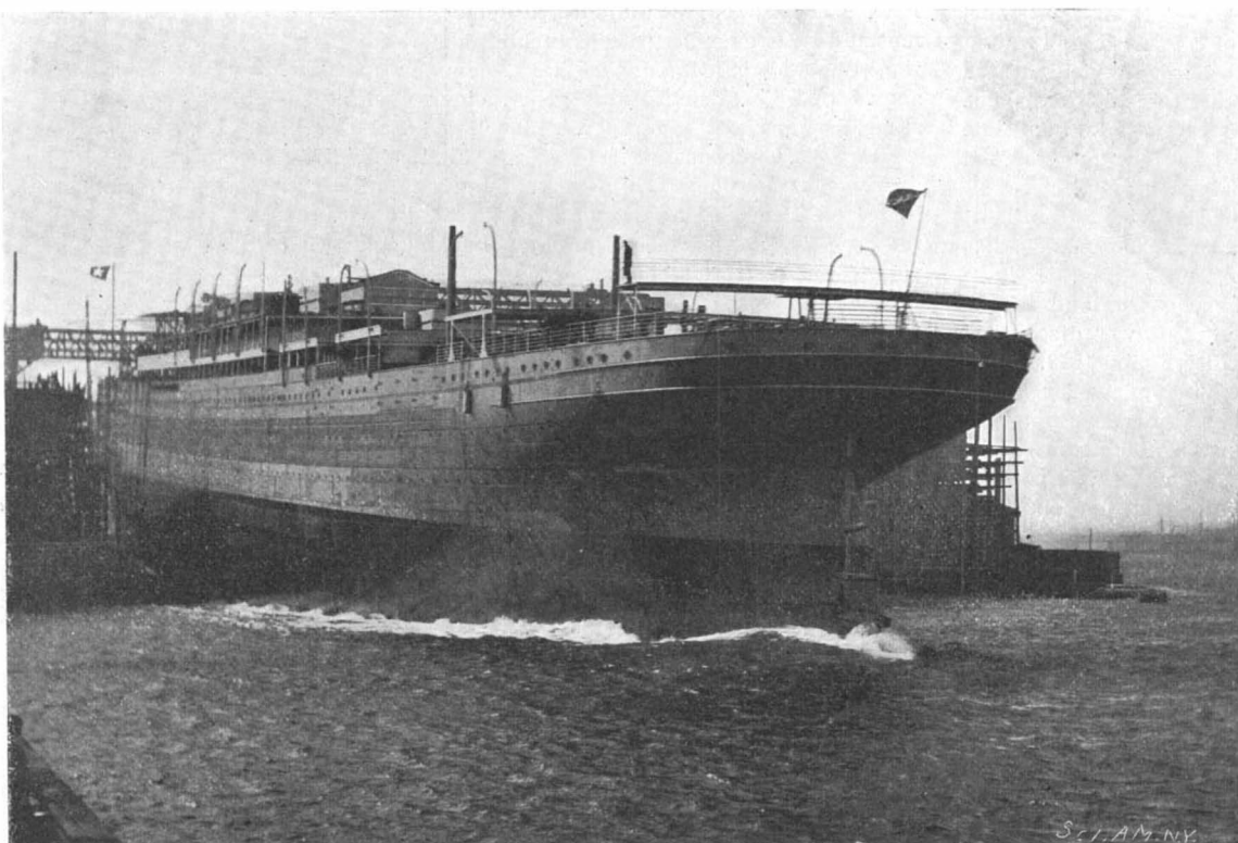
Length, 700 feet; beam, 75 feet; depth, 49 feet; maximum displacement, 37,700 tons; Speed, 16¼ knots.
