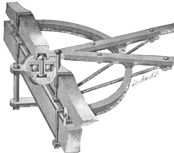
THE BURDICK FIFTH-WHEEL FOR WAGONS AND CARRIAGES.
