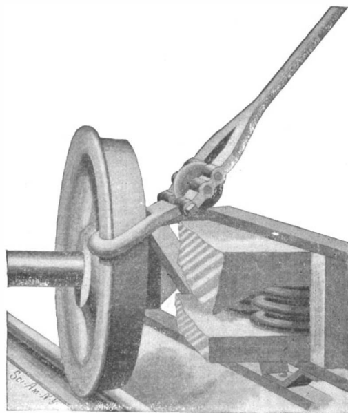
KURTZ'S CAR-MOVER.
