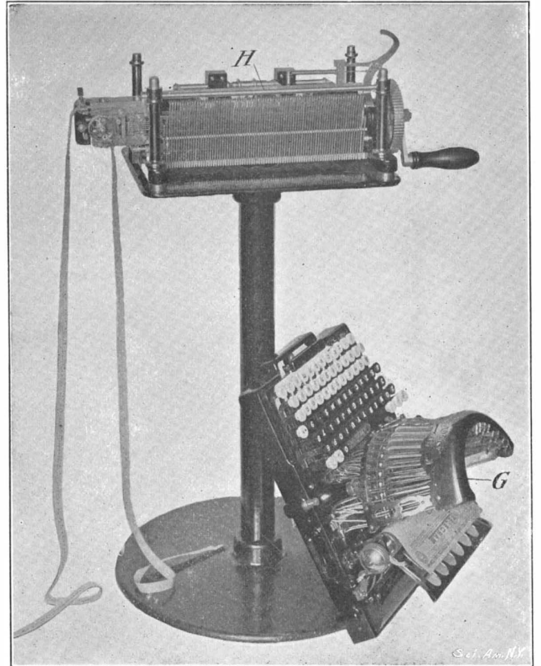
The typewriter, G, is removed to show the interlocking mechanism, H, by which the perforated characters on the tape are made to strike the keys of the Roman alphabet on the typewriter.
