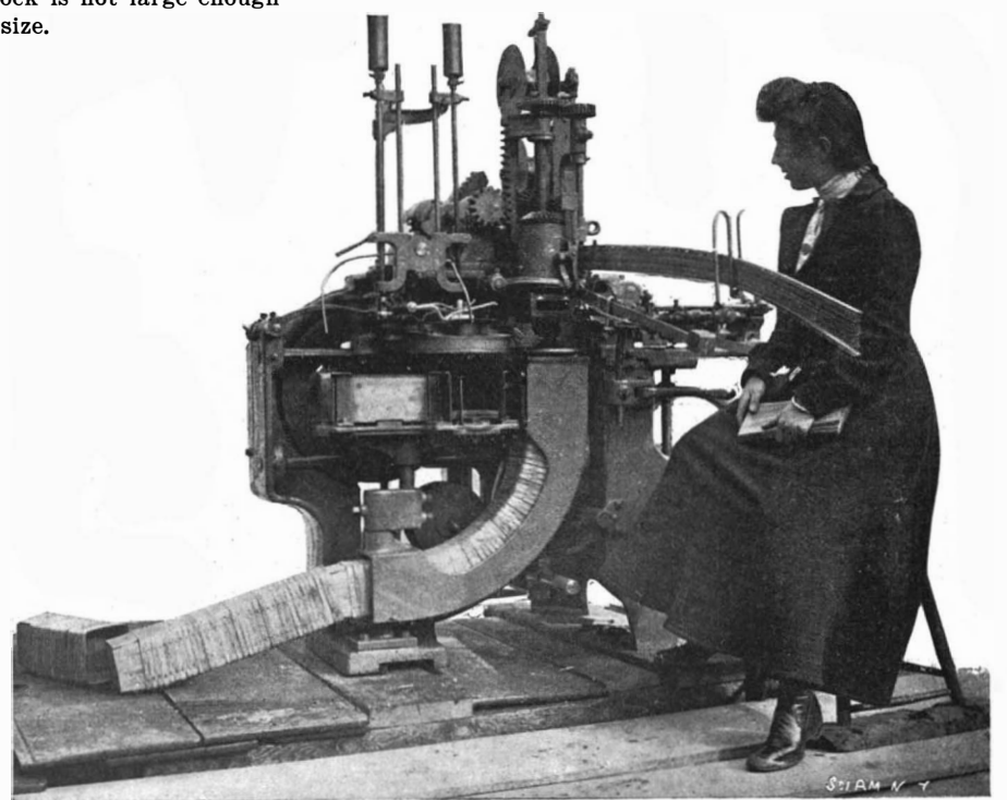
HORTON BERRY-BASKET MACHINE.
