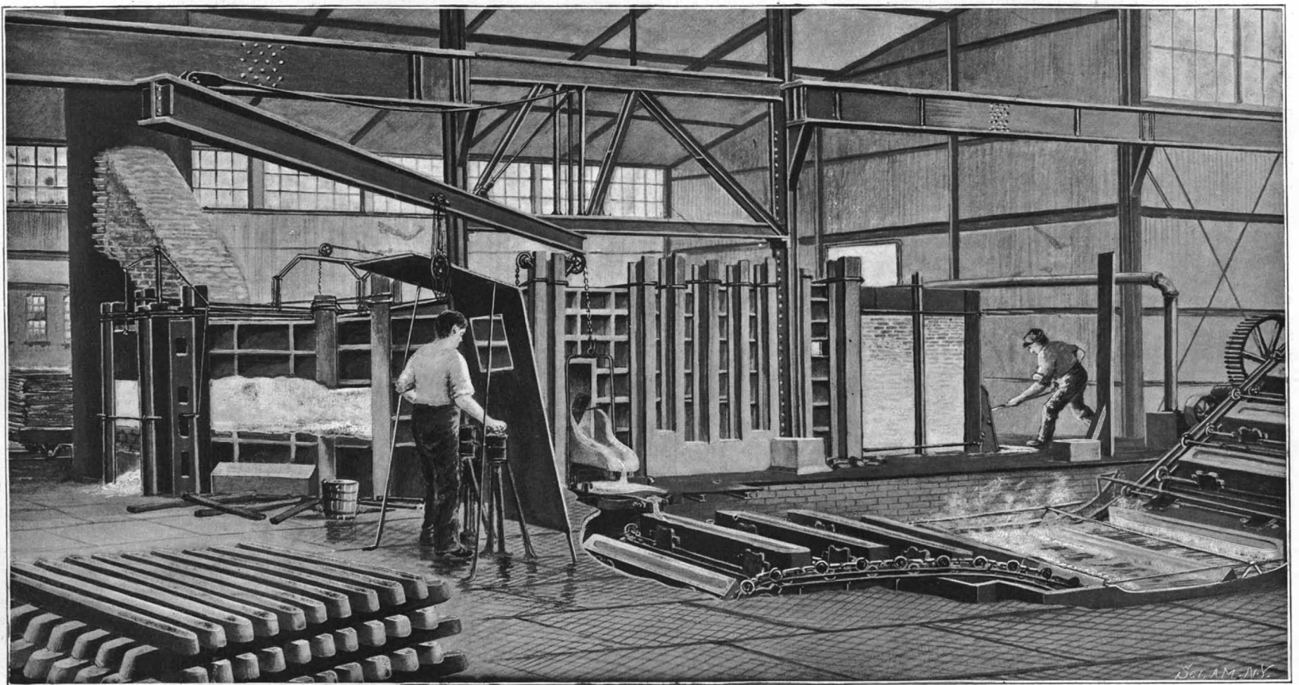
The Furnace House—Casting and Cooling Refined Copper Bars. THE ELECTROLYTIC REFINING OF COPPER.—[See page 187.]
