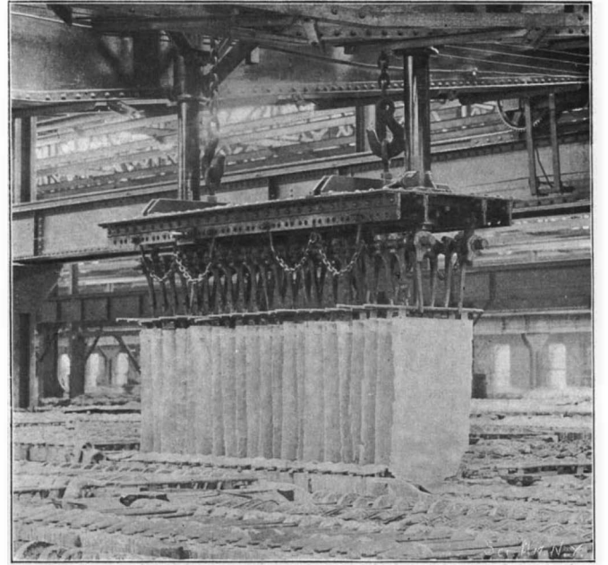
Traveling Crane Placing Set of Cathode Plates in a Tank.
