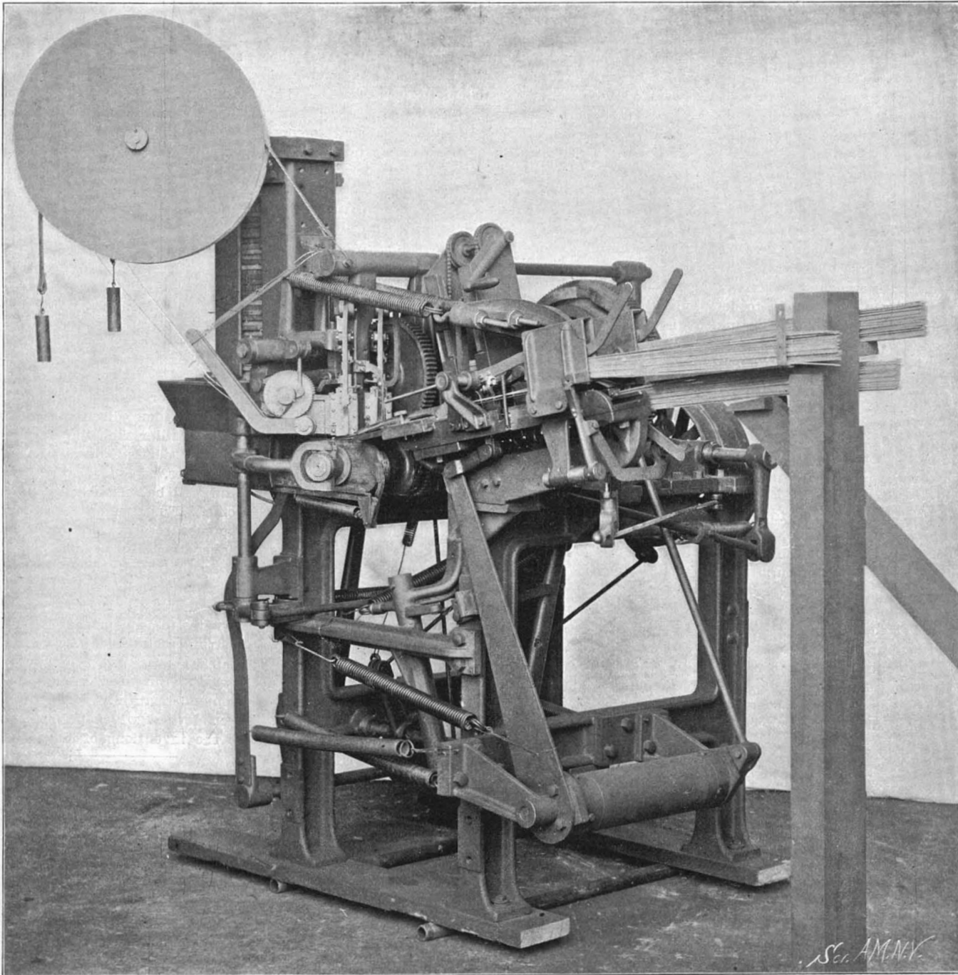
MERGENTHALER GRAPE BASKET MACHINE.
