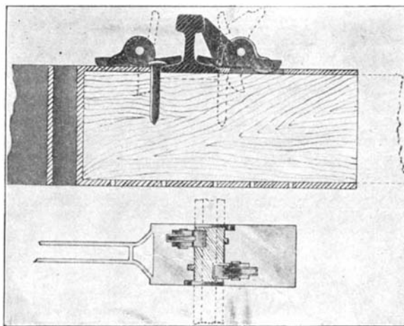
METAL CROSS TIE FOR RAILROADS.
