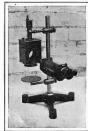
Fig. 2.—General View of the Electroscope.
