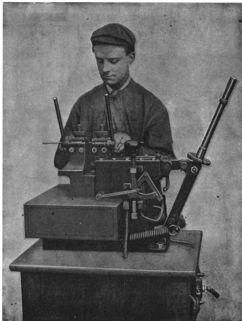
AN IMPROVED ELECTRIC WELDER.
