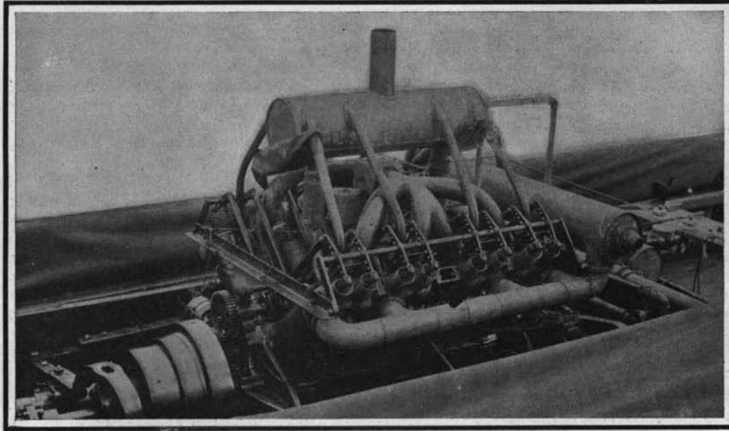
Cooper Hewitt's 8-Cylinder Motor Installed in the Hull of His Gliding Craft.
