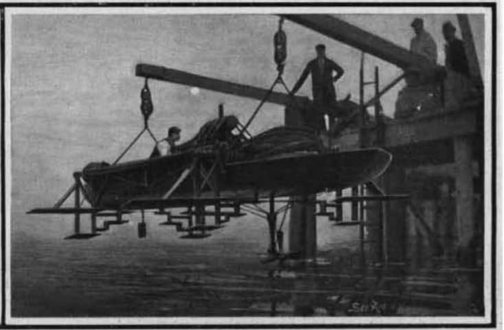
The Hydroplanes and Propeller Below the Hull.
