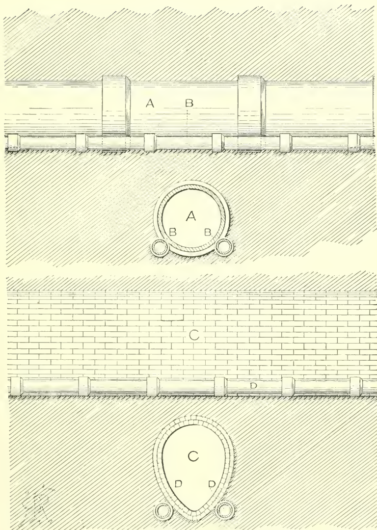
PLATE 20. DRAINAGE & SEWER SYSTEMS SEPARATED.
