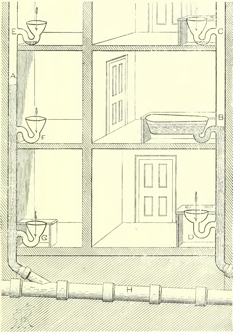
PLATE 13 - SIPHONING TRAPS
