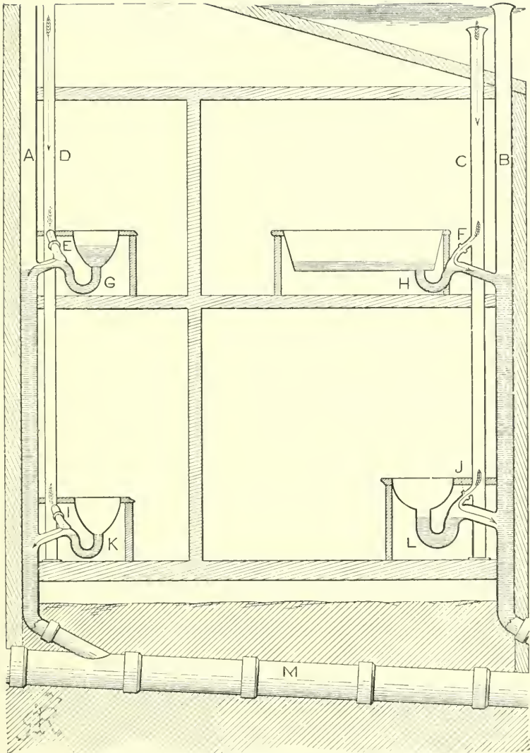
PLATE 14 - NON-SIPHONING TRAPS
