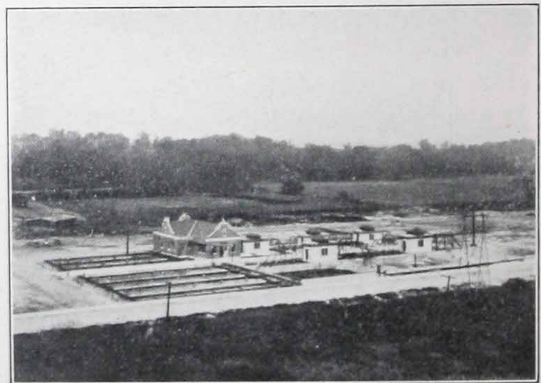
ACTIVATED SLUDGE PLANT AT YORK TOWNSHIP, ONT. Showing Dorr Clarifiers at right. Dorr equipment is operating in many sewage plants in Canada
