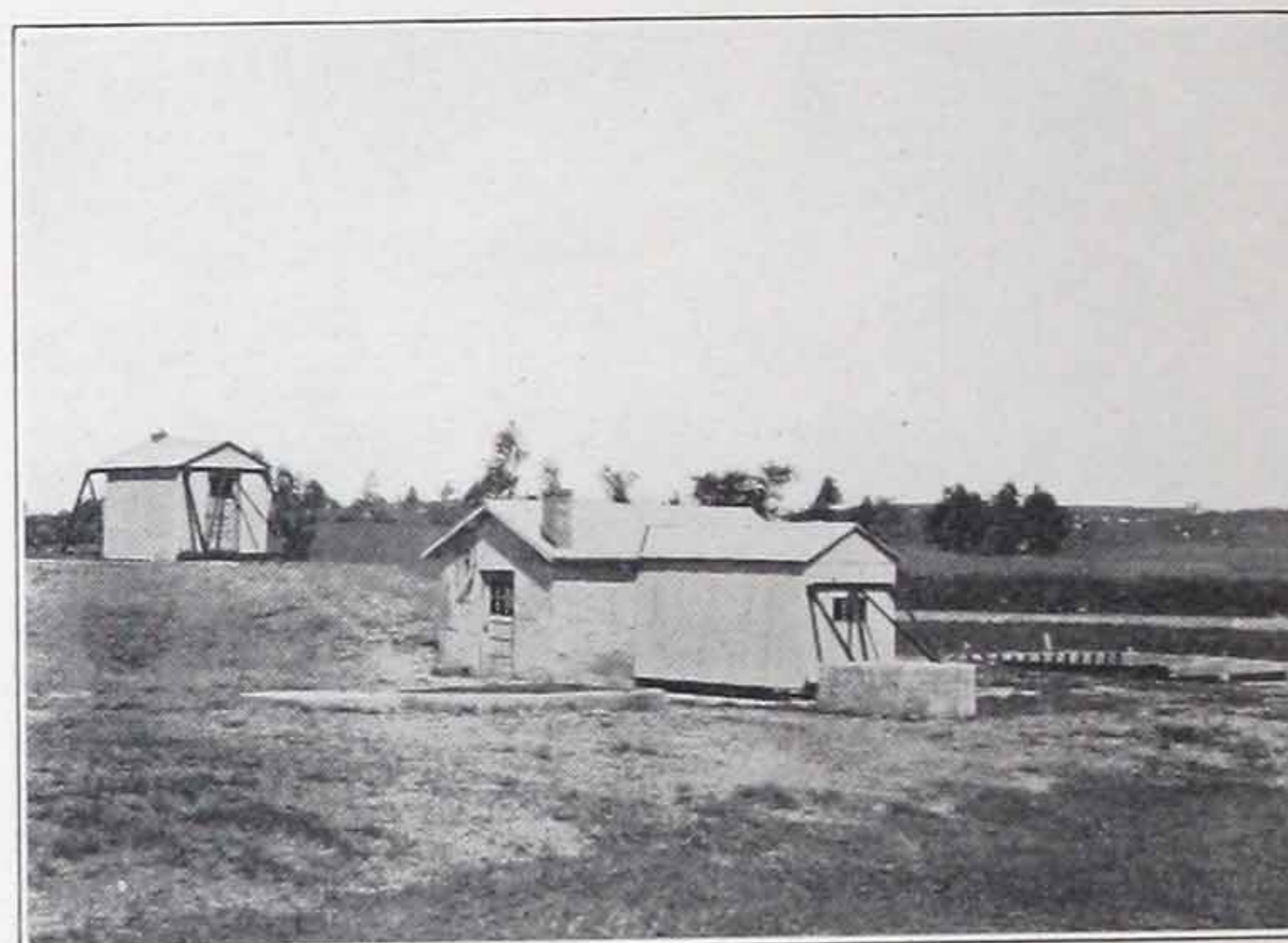
SEPARATE SLUDGE DIGESTION PLANT AT KIEL, WIS. The Clarifier is at right of photo, while the Dorr Digester is seen at the left
