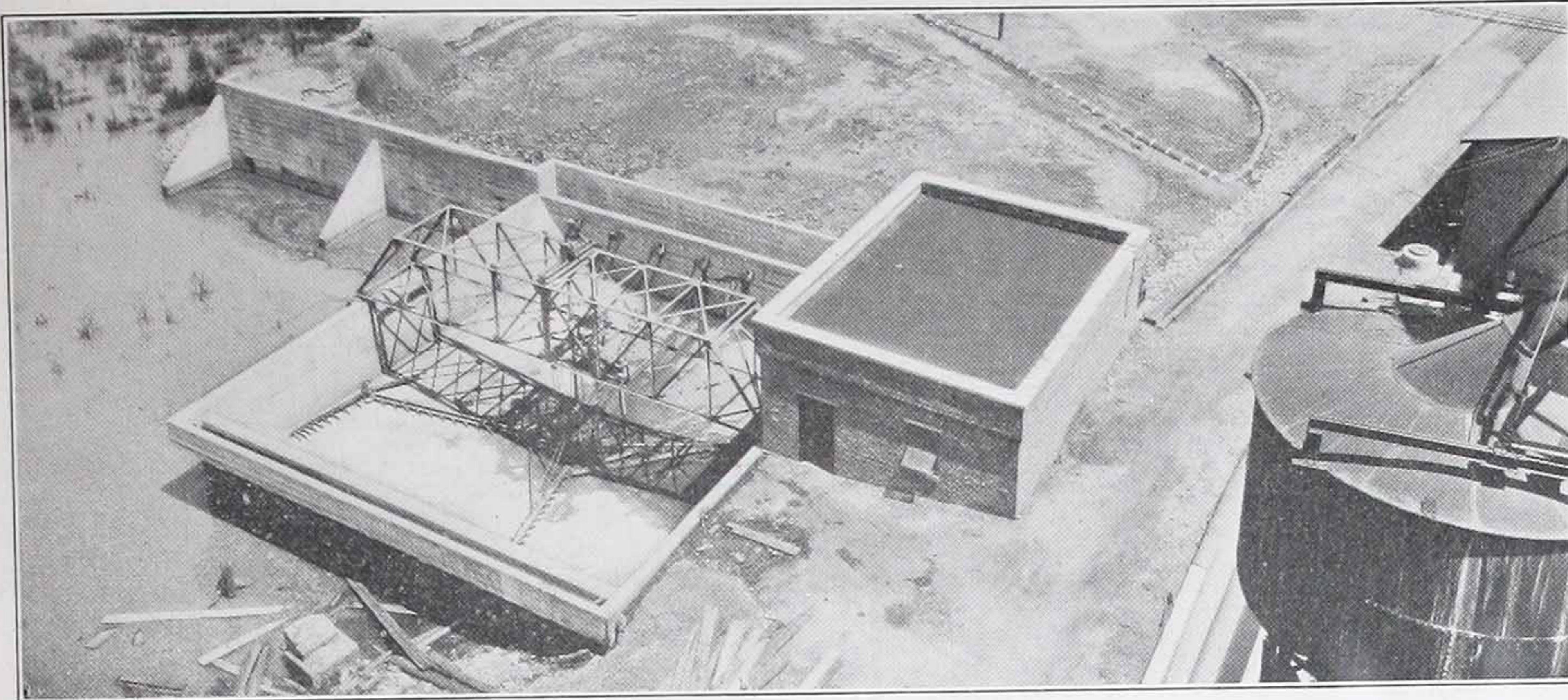
WASTE TREATMENT PLANT OF THE STANDARD BLEACHERY CO., CARLTON HILL, N. J.
