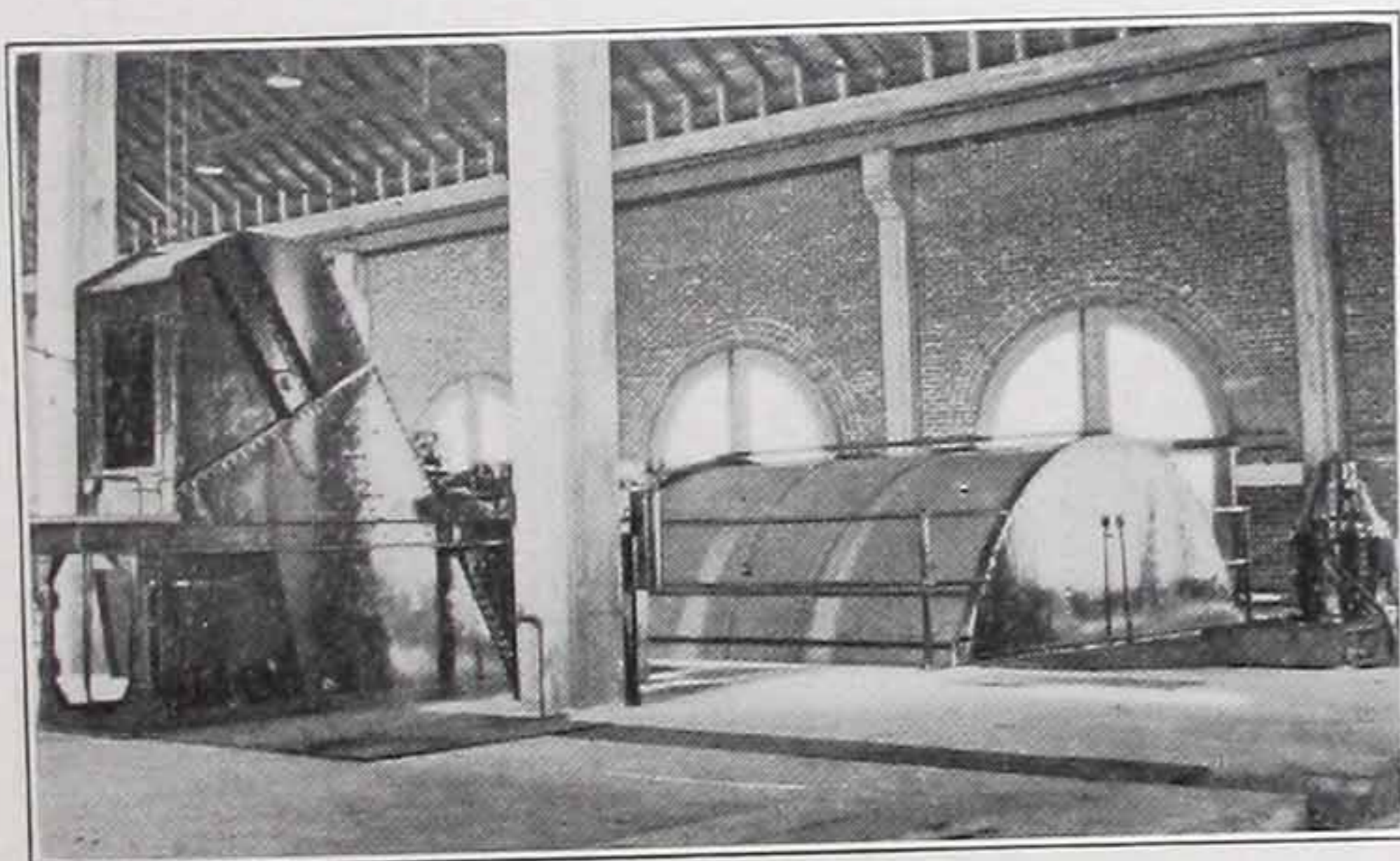
ONE OF THE FIVE 14' x 12' DORRSCO SCREEN UNITS IN THE NORTH HYPERION PLANT, LOS ANGELES
