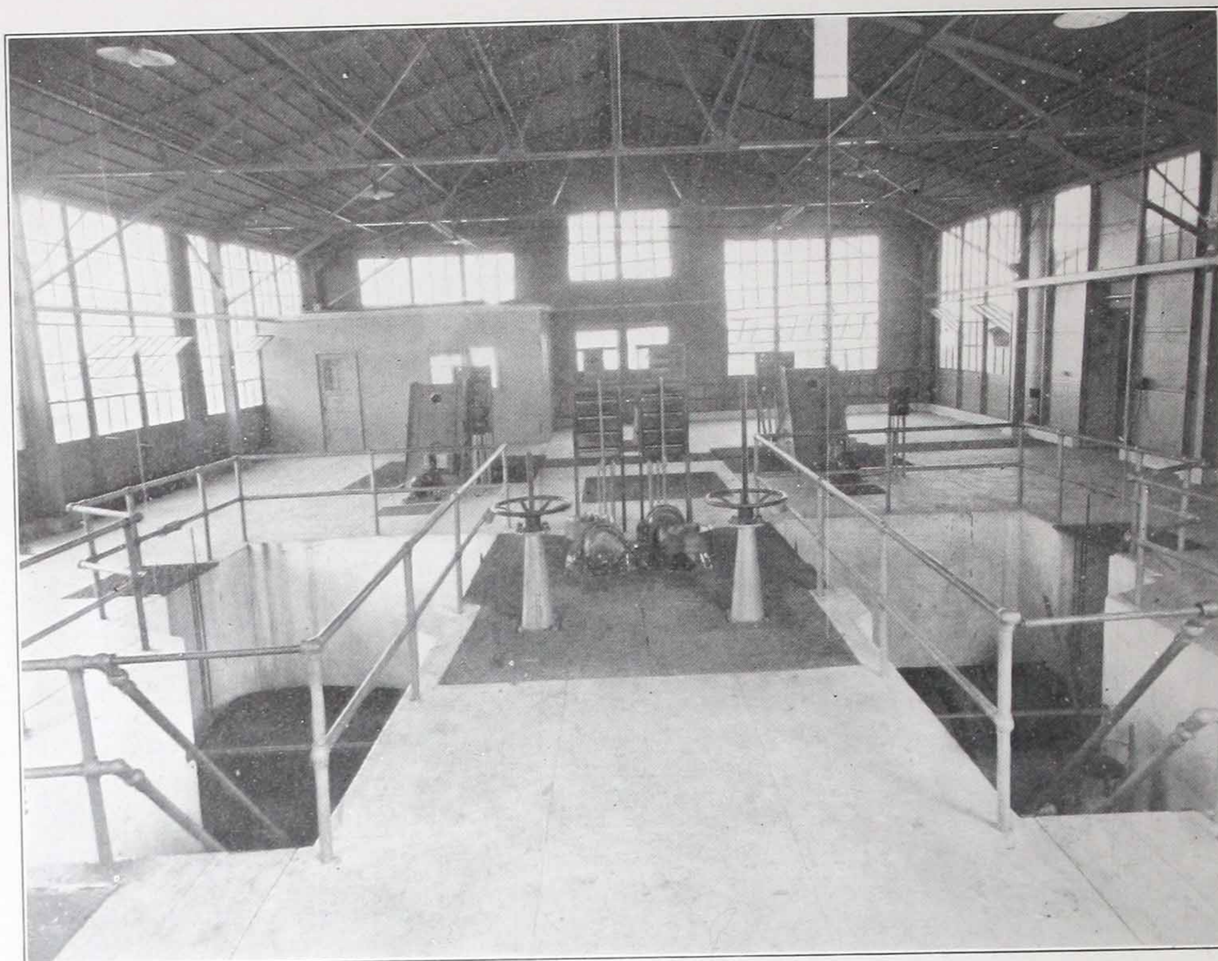
INTERIOR OF SCREENING PLANT AT LONG BEACH, CAL., SHOWING THE TWO DORRICO SCREEN UNITS
