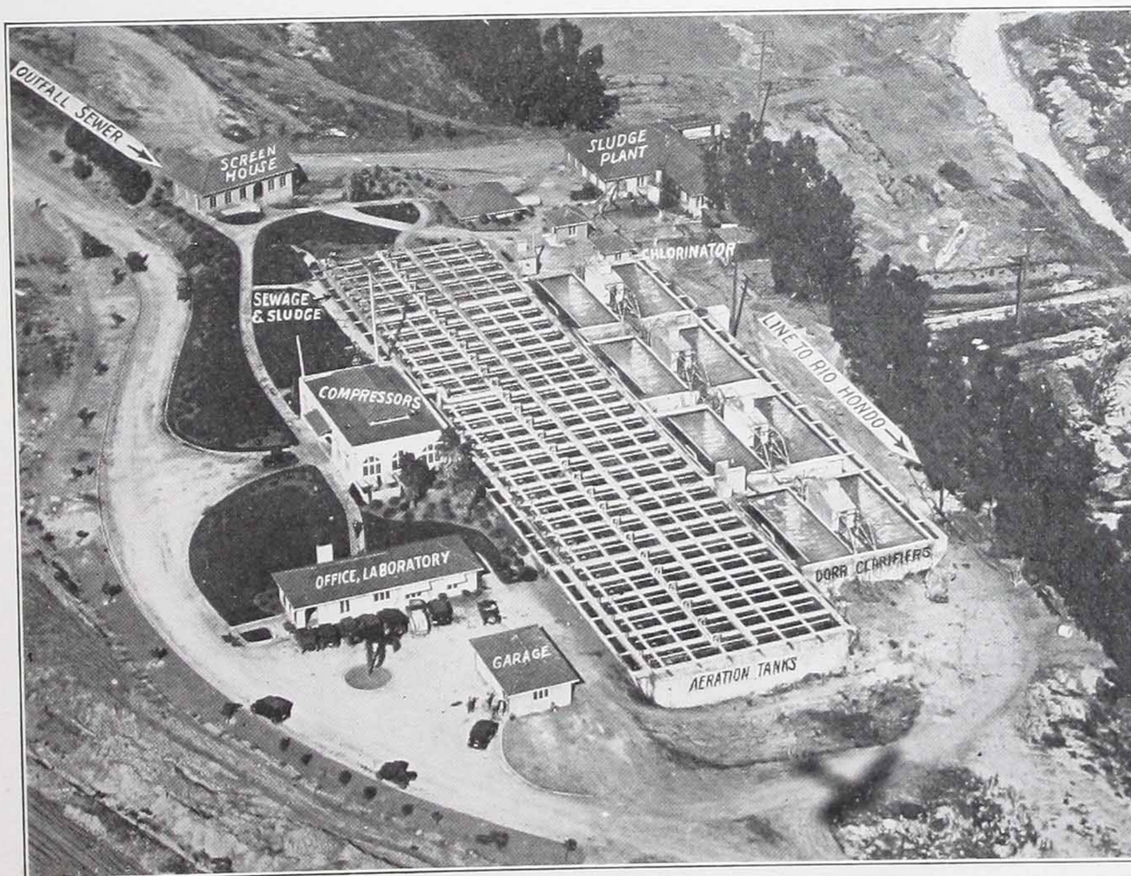
GENERAL VIEW OF ACTIVATED SLUDGE SEWAGE DISPOSAL PLANT, PASADENA, CAL.
