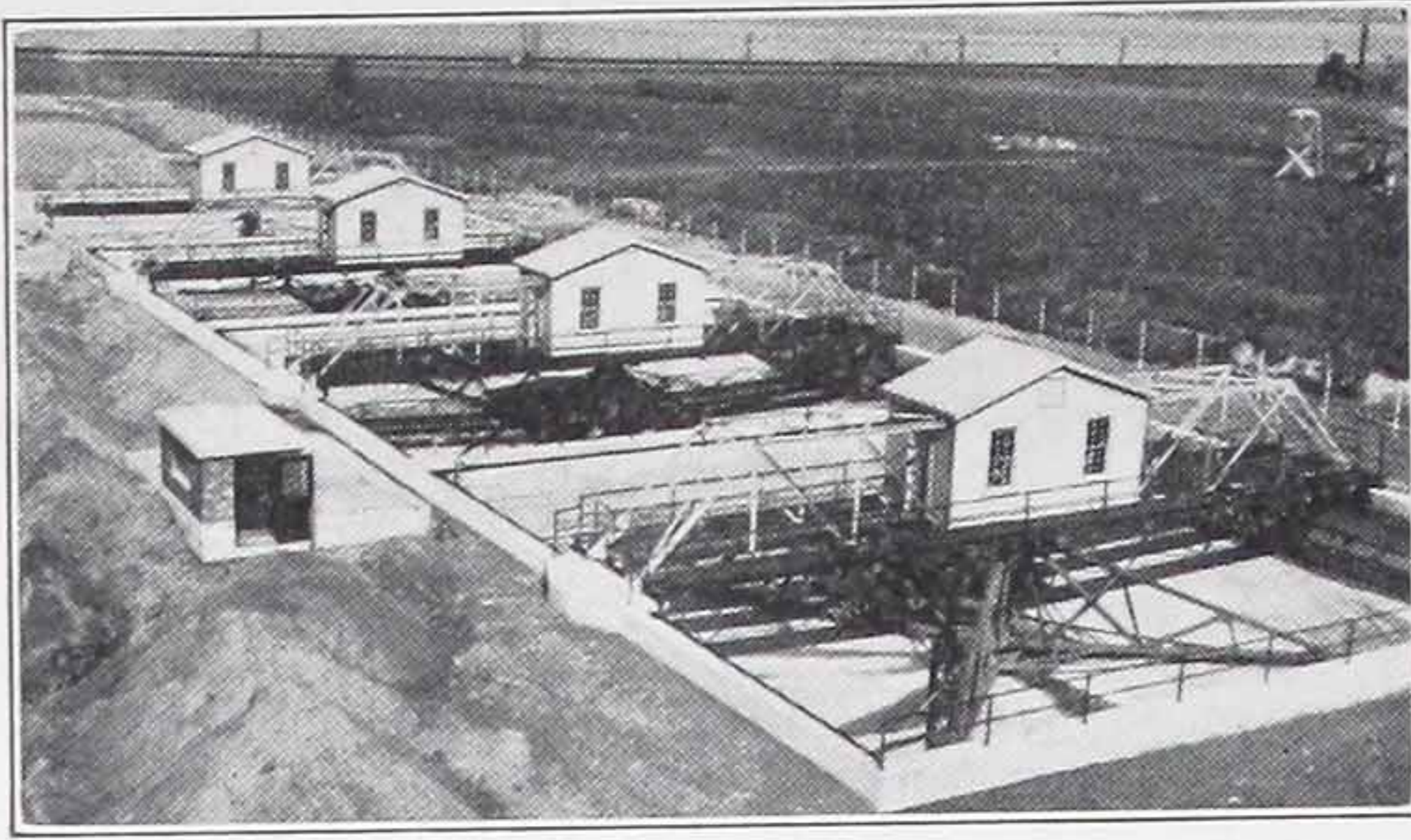
FOUR 71-FOOT DORR CLARIFIERS IN THE SEWAGE TREATMENT PLANT, SYRACUSE, N. Y.
