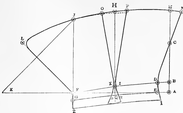
STORM COLLAR
