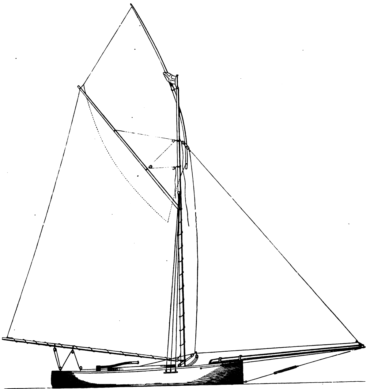
Sail Plan of Windermere Yacht.
