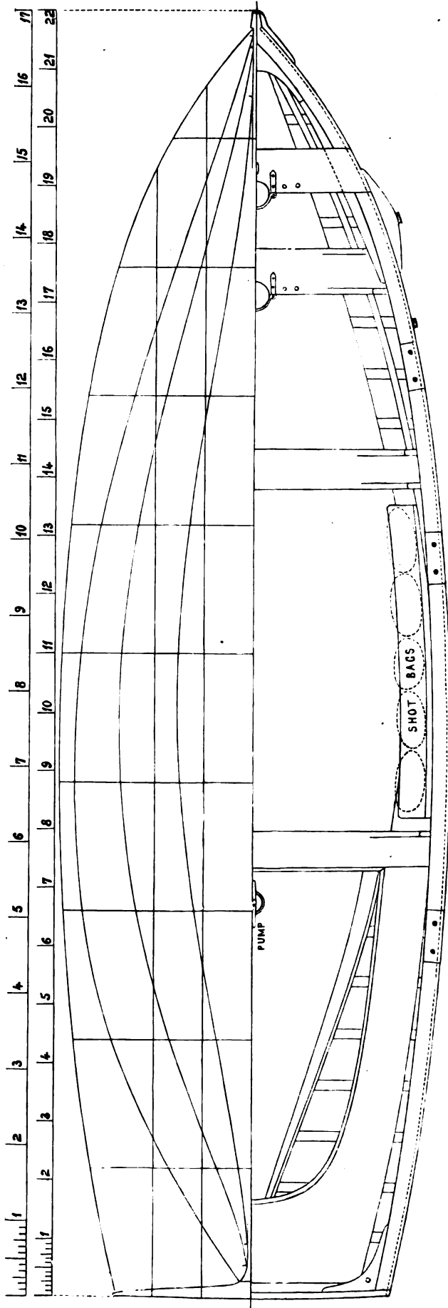
Clyde Sailing Boat—General Plan.
