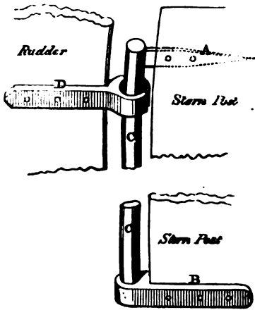
\frac{1}{2} Full Size FIG. 146.
