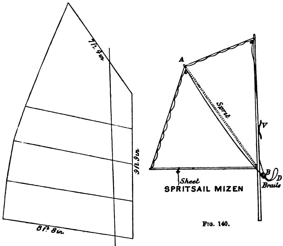
RACING MAINSAIL. \frac{1}{8} INCH SCALE.
