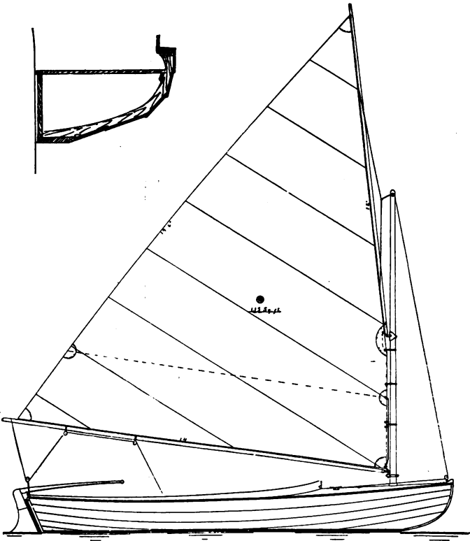
A 16-FT. LAP STRAKE CATBOAT
