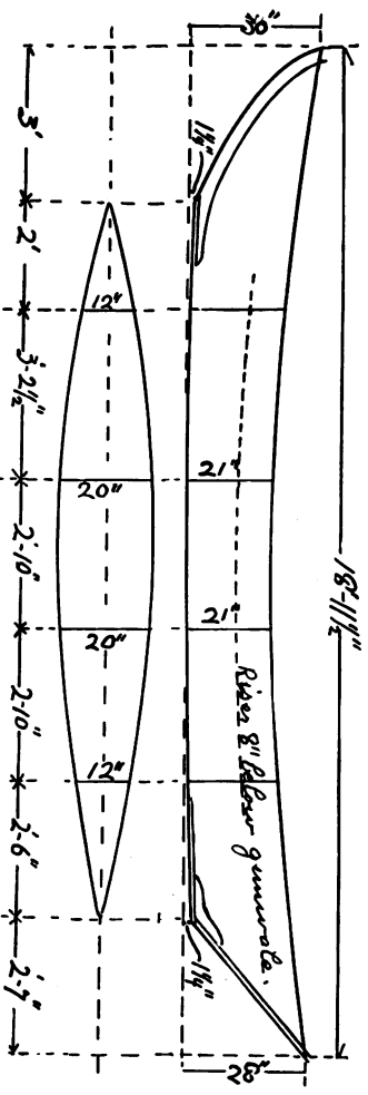
Fig 2.—Construction plan, with all necessary measurements from which to cut paper patterns
