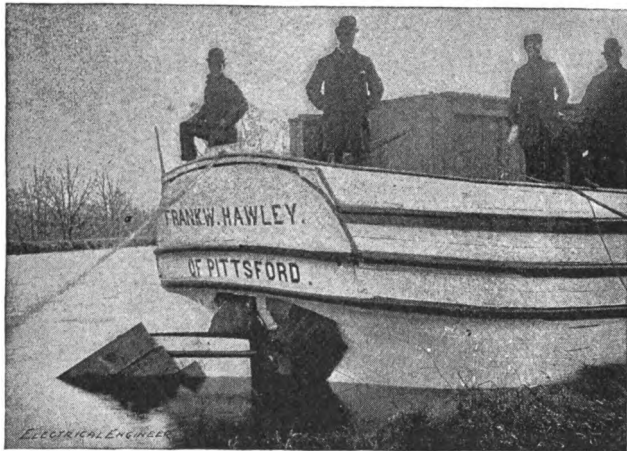
FIG. 51a.—PROPELLER OF THE “FRANK W. HAWLEY.”
