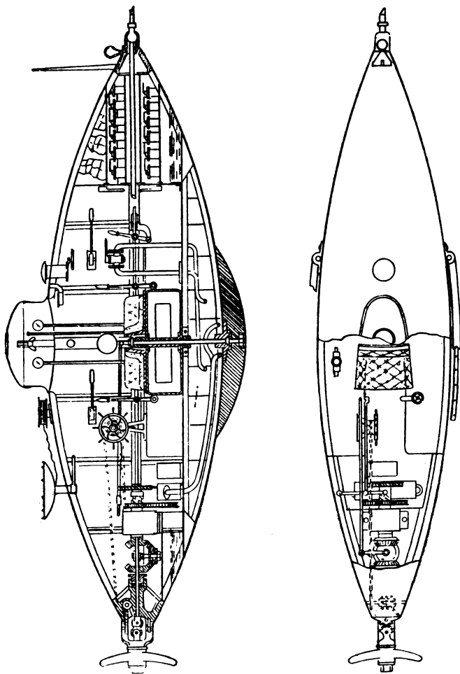
FIGS. 36 AND 37.—THE "GOURET" ELECTRIC BOAT.
