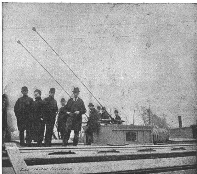
FIG. 51C.—DECK OF THE "FRANK W. HAWLEY," SHOWING THE TROLLEY POLES.
