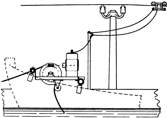
FIG. 61.—BUSSEK METHOD OF SUBMERGED FLEXIBLE CABLE HAULAGE.
