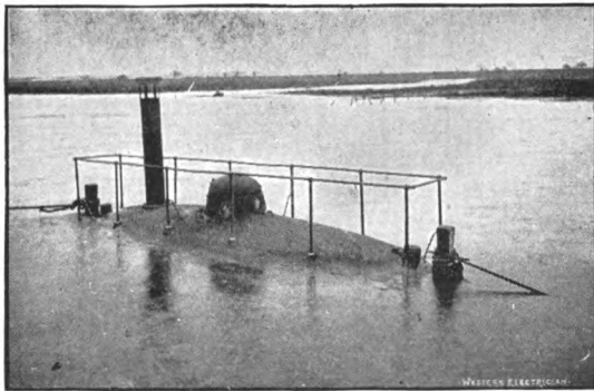
FIG. 39.—APPEARANCE OF BAKER BOAT WHEN READY FOR GOING UNDER WATER.
