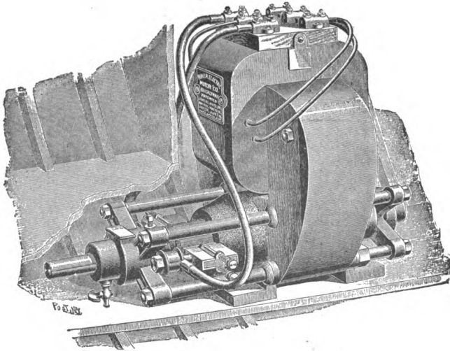
FIG. 13.—MOTOR OF RIKER ELECTRIC LAUNCHES.
