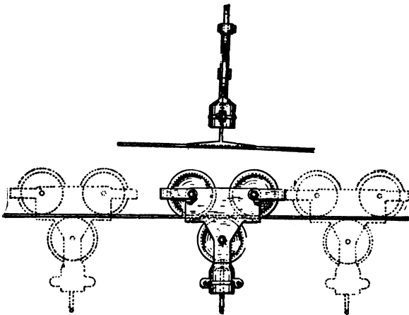
- FIG. 52a.—LATERALLY MOVABLE TROLLEY WIRE AND HANGER.
