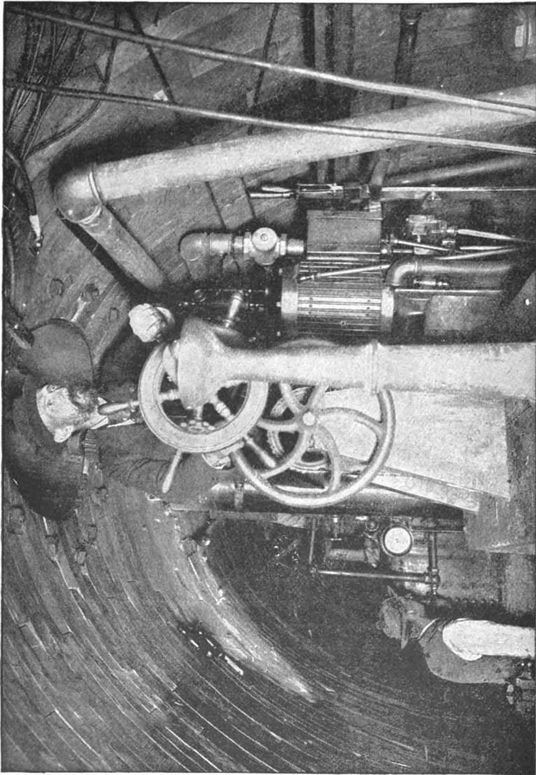
FIG. 39a.—INTERIOR OF BAKER BOAT WHEN IN OPERATION UNDER WATER.
