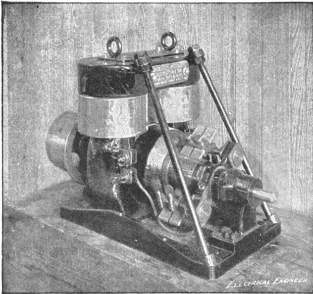
FIG. 21.—CROCKER-WHEELER ELECTRIC LAUNCH MOTOR.
