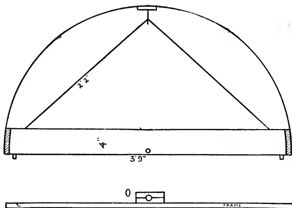
Fig. 5 SHOWING CONSTRUCTION OF PADDLE-BOX O, crank-bearing fastened to frame, as shown in Fig. 2
