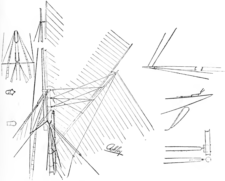
HINTS ABOUT RIGGING, ROPES, BLOCKS, STAYS, AND SHROUDS
