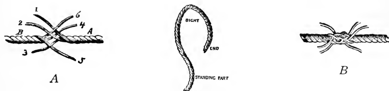
FIG. 2. THE SHORT SPLICE
