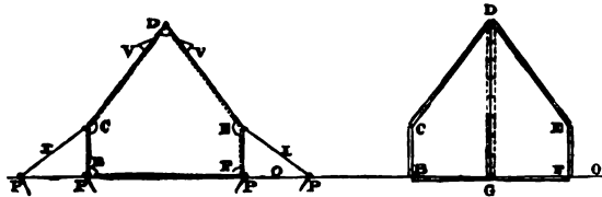
Back Elevation. Scale 1"=1ft. FIG. 172.
