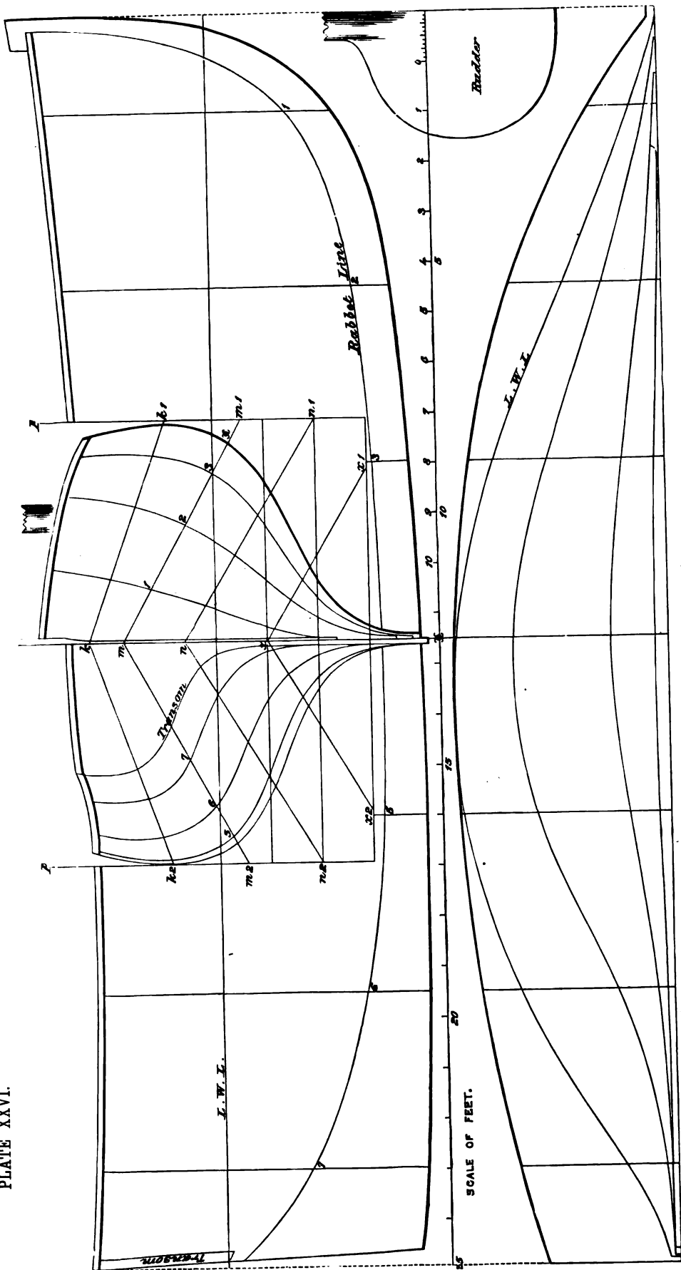
Itchen Boat "Wild Rose," 25ft.
