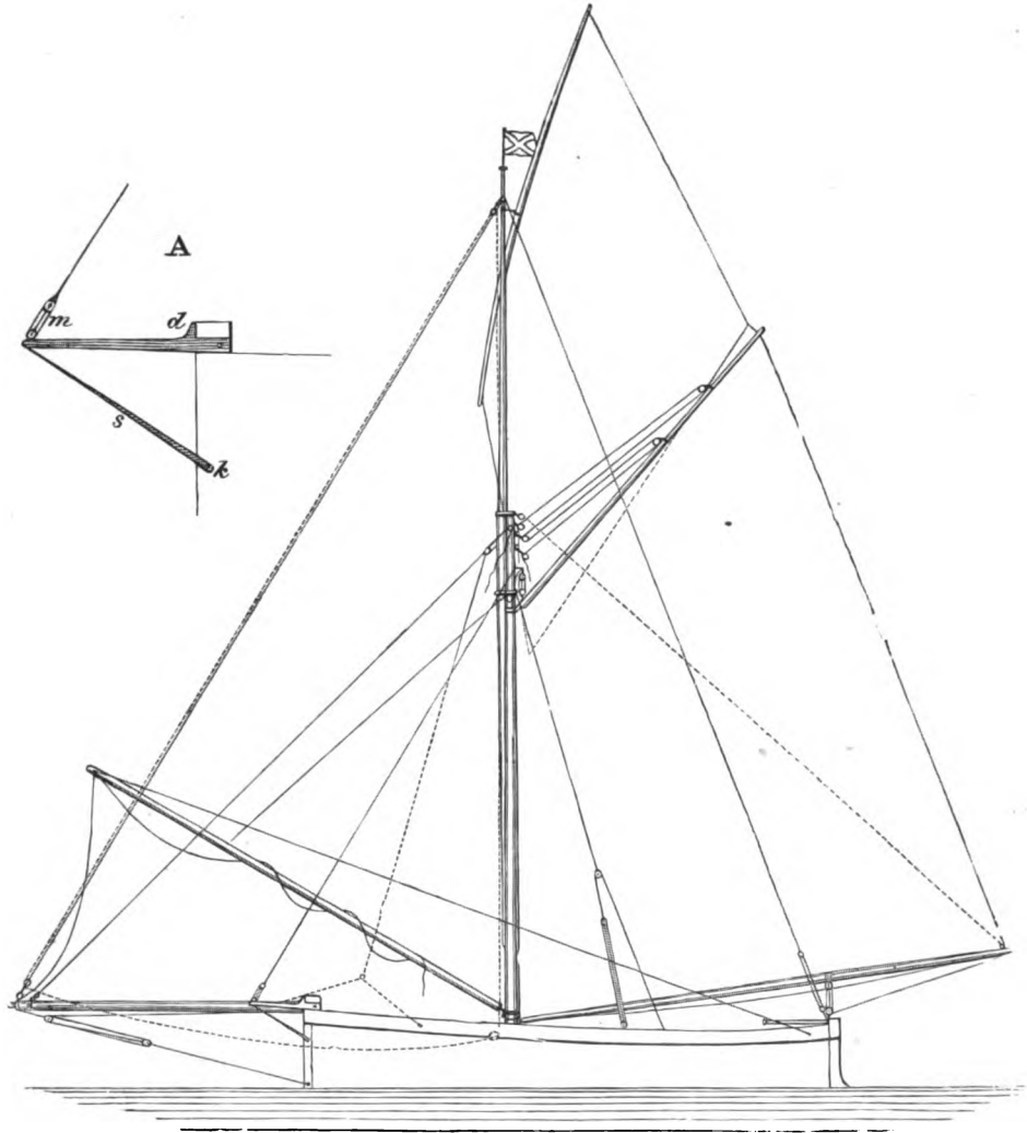
ITCHEN BOAT. SCALE \frac{1}{2} = 1 FOOT.
