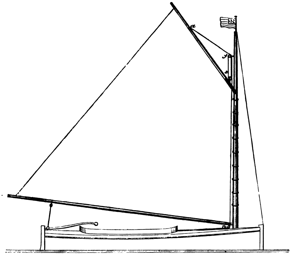
SAIL PLAN "UNA" BOAT 4" INCH SCALE.
