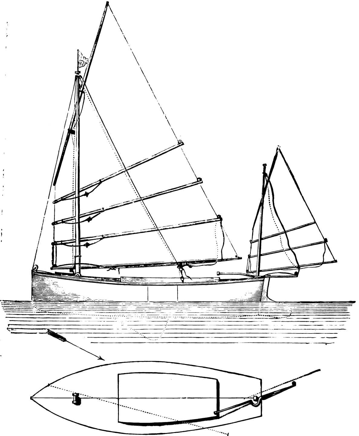
Chinese Lug Sail : Main and Mizzen Rig.
