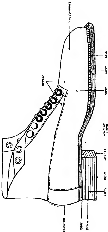
FIG. 10.—External parts of the shoe.
