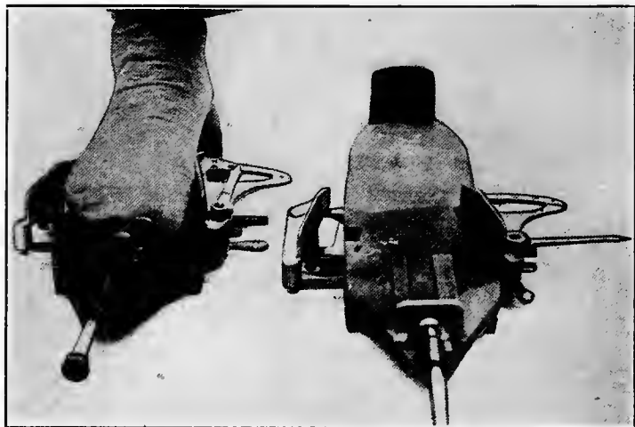
FIG. 36.—Foot being measured in Resco marine corps foot measuring device.
