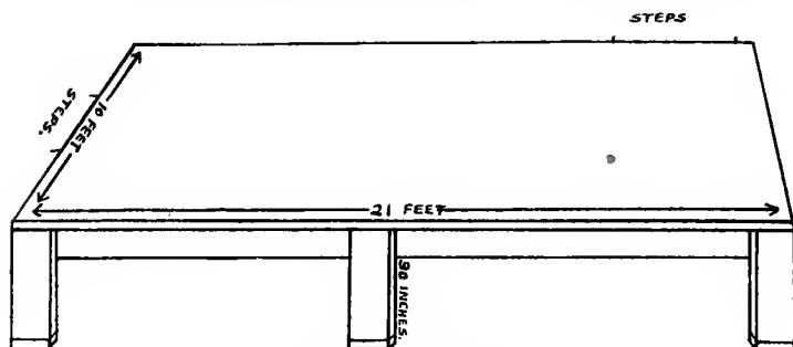
FIG. 42.—Measuring platform.
