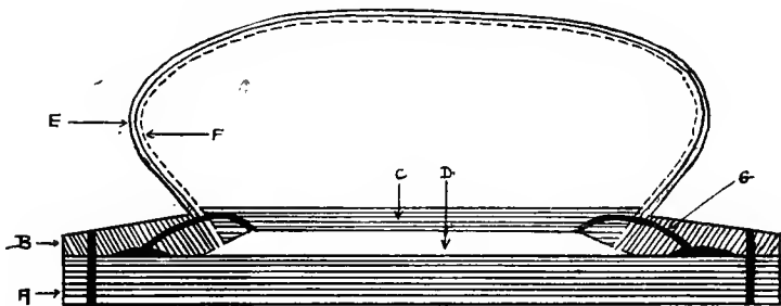
FIG. 11.—Goodyear welt shoe. Cross section. Sole, welt, insole and fill exaggerated.
