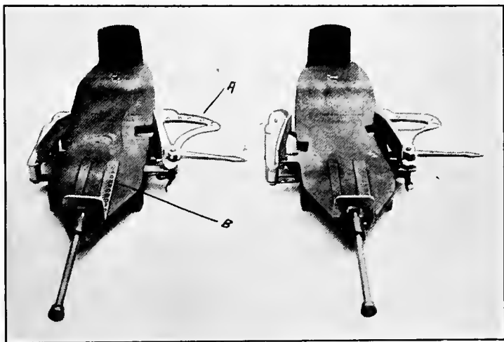
FIG. 34.—Resco marine corps foot measuring device.
