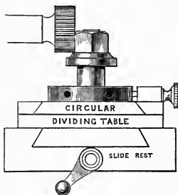
COLLAR-NUT CUTTING MACHINE.
