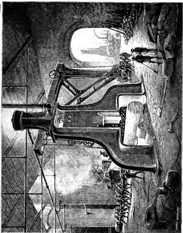
STEAM HAMMER IN FULL WORK. FROM A PAINTING BY JAMES NASMYTH.
