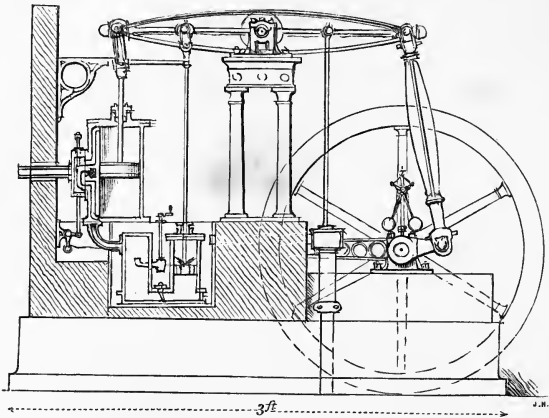
SECTIONAL MODEL OF CONDENSING STEAM-ENGINE. BY JAMES NASMYTH.
