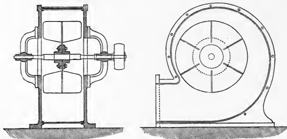
1845. A Direct Action "Suction" Fan for the Ventilation of Coal-Mines.
