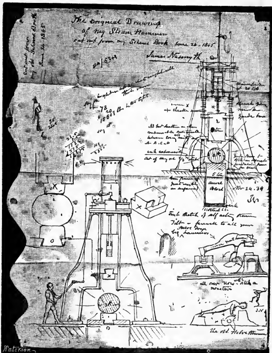
FIRST DRAWING OF STEAM HAMMER, 24TH NOV. 1839.
