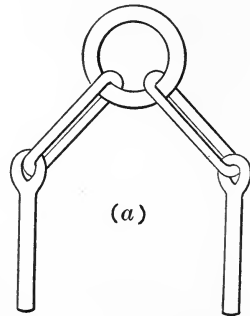
FIG. 74.—Dowels for Lifting Cut Stone. (a) Pin Lewis; Capacity, 1,000 to 6,000 Pounds.
