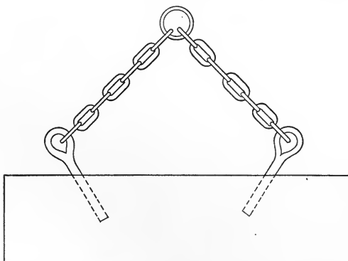
FIG. 74.—Dowels for Lifting Cut Stone. (a) Pin Lewis; Capacity, 1,000 to 6,000 Pounds.
