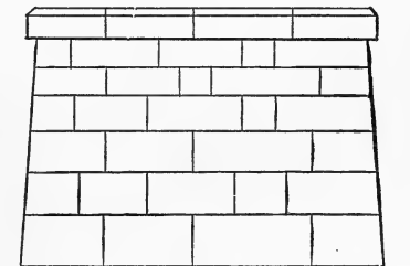
FIG. 60.—Irregular Coursed Ashlar, Courses Have Different Heights.
