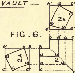
— SKETCH OF VAULT —
