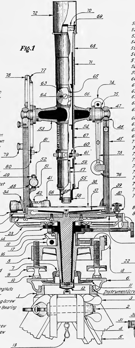
Cross section of the Berger Transit.
