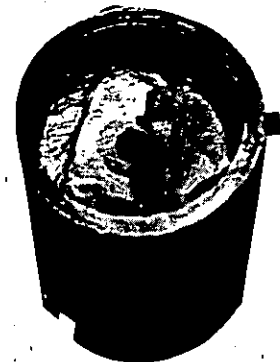
The 1 1/2" steel pipe piece dropped in breech as spacer, with firing pin washer dropped in on top of welded washer-spacer and second washer.
