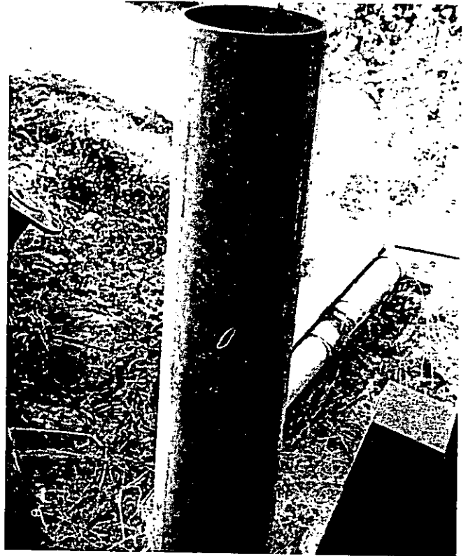
Constructing a claymore by sawing out the back blast shield. Use a 1/3 section of heavy-duty (1/4-inch side wall) PVC pipe. Mark the rim of the pipe off in three equal (9-inch) segments.
