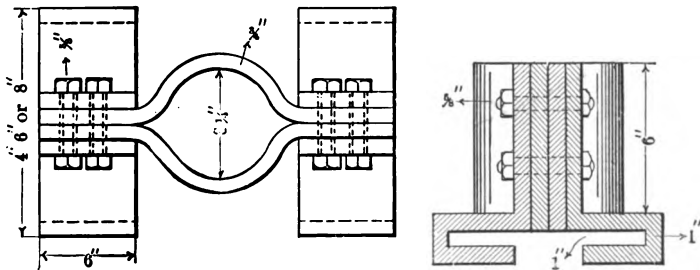
FIG. 141.— POLE BASE FOR IRON ROOF.
