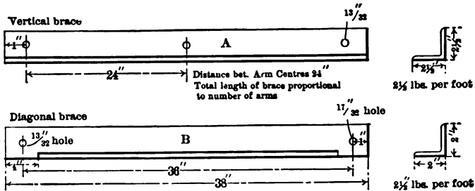
FIG. 64.—ALLEY ARM BRACES.
