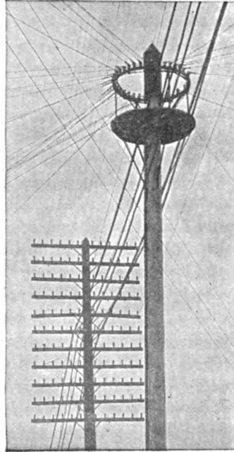
FIG. 31.— POLE TOP WITH PLATFORM.
