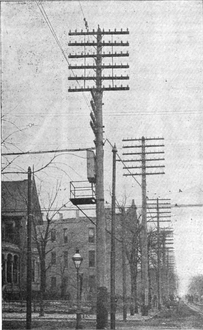
FIG. 3.—POLE LINE IN CHICAGO.
