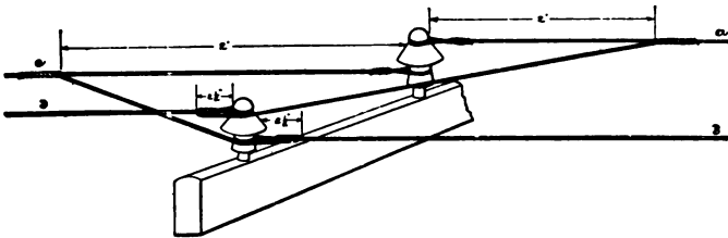
FIG. 128.—RECENT METHOD OF MAKING TRANSPOSITIONS.
