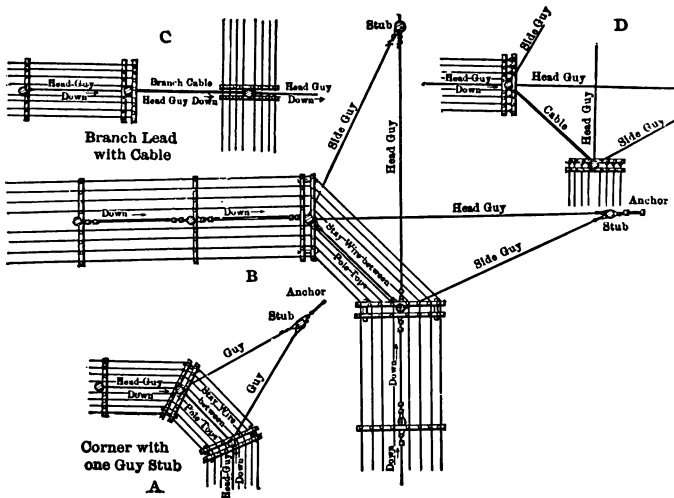
FIG. 107.— CURVE AND CORNER DETAILS.
