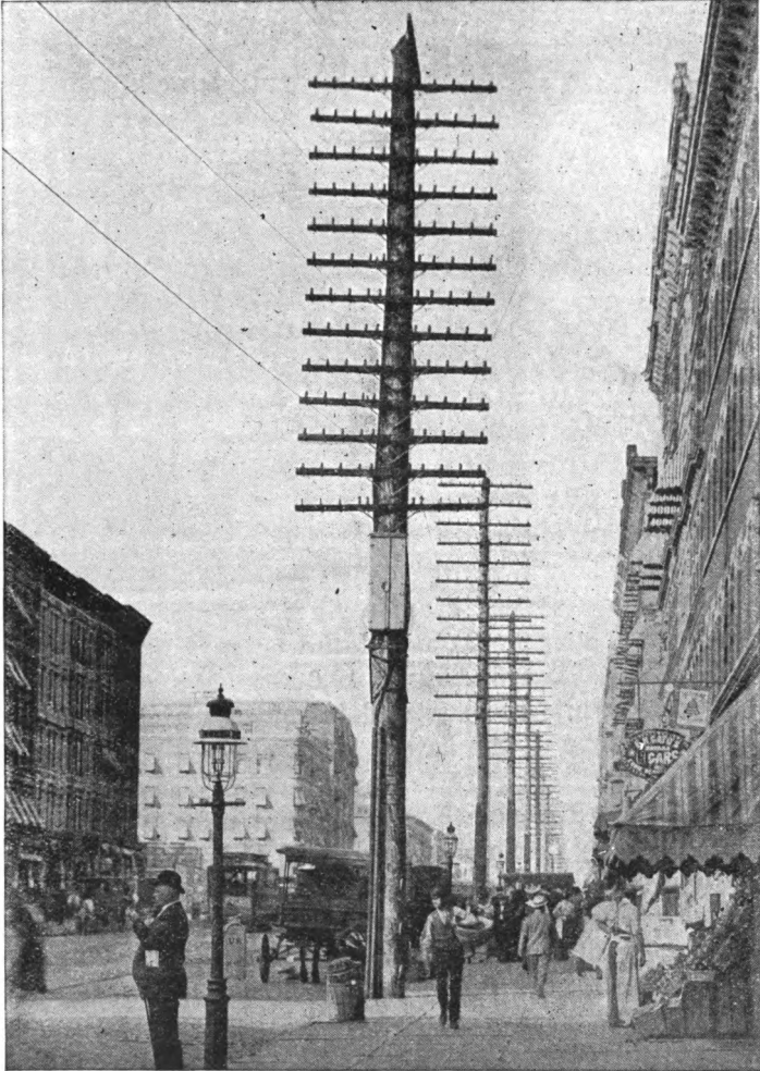
FIG. 1.—POLE LINE — AMSTERDAM AVENUE, NEW YORK.
