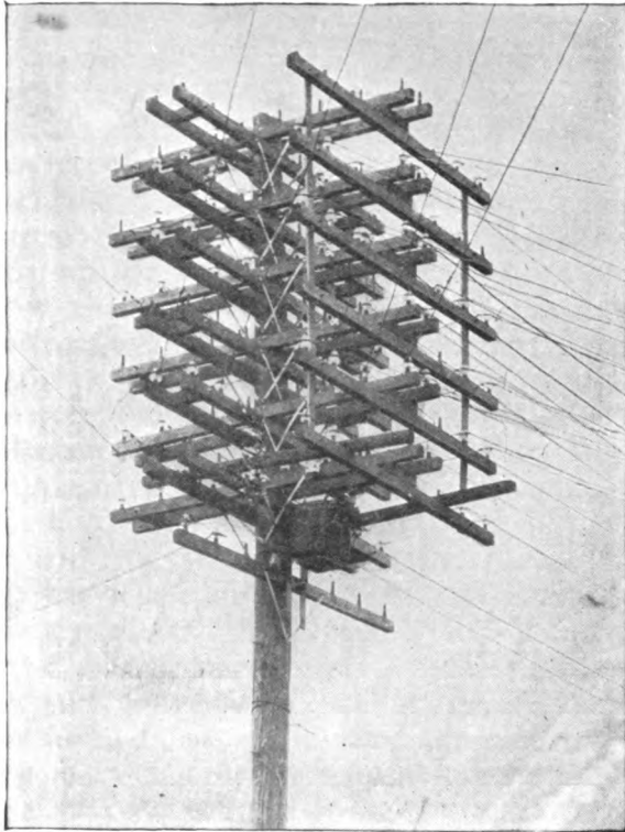
FIG. 93.— EXAMPLE OF DOUBLE ARMING.
