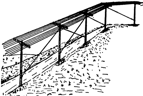
FIG. 102.— HEAD GUYING TO LINE.
