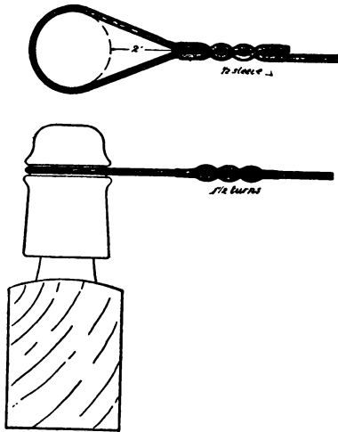
FIG. 123.—METHOD OF DEAD-ENDING.
