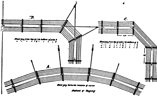
FIG. 106.— CURVES AND CORNERS.
