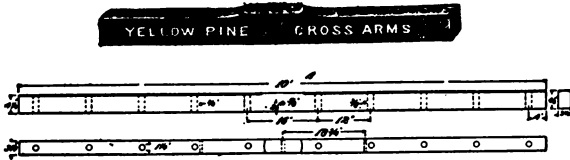
FIG. 53.—YELLOW PINE CROSS ARMS.
