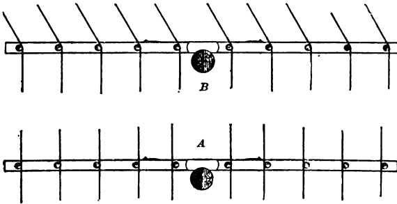
FIG. 117.—LOCATION OF WIRE ON PINS.
