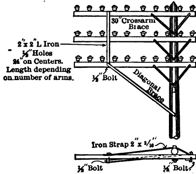
FIG. 54.—ALLEY ARM LOCATION.
