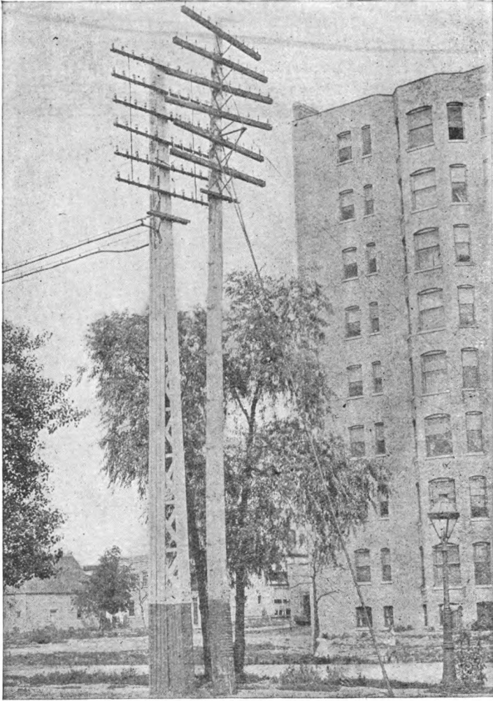
FIG. 22.—STRUCTURAL IRON POLE.
