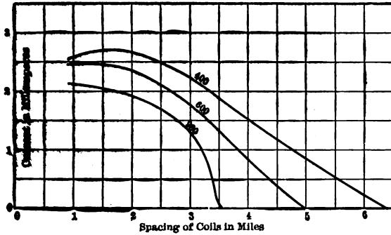
FIG. 8.— CURVES SHOWING RELATION BETWEEN NUMBER OF COILS PER MILE AND CURRENT TRANSMITTED.
