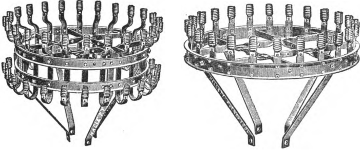
FIG. 37.—DETAILS OF CHANNEL IRON POLE TOP.
