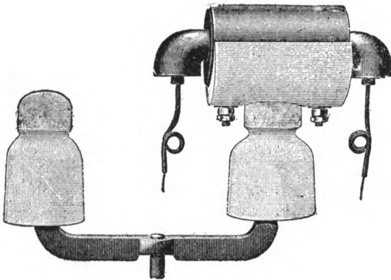
FIG. 5.— AERIAL LINES — COMPENSATING COILS.
