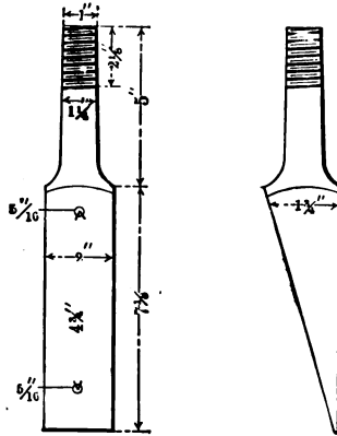
FIG. 51.— WOOD BRACKET.
