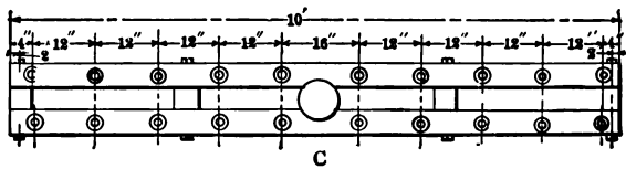
FIG. 92 C.—DOUBLE ARMING.
