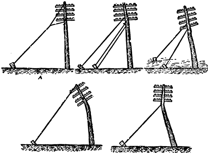
FIG. 21.—WRONG METHODS OF GUYING.
