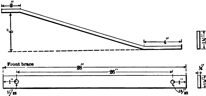
FIG. 63.—BACK CROSS-ARM.
