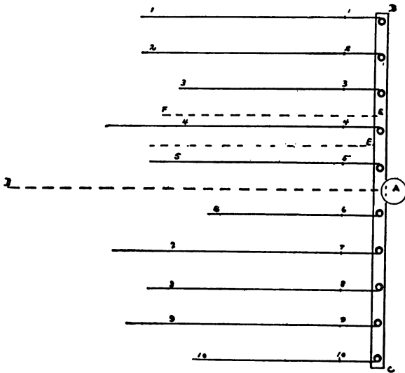
FIG. 17.—PLAN OF POLE LINE.
