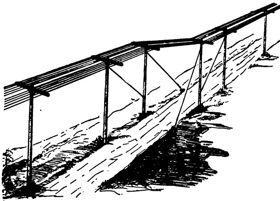
FIG. 110.— HIGHWAY CROSSING WITH SIDE GUYS.
