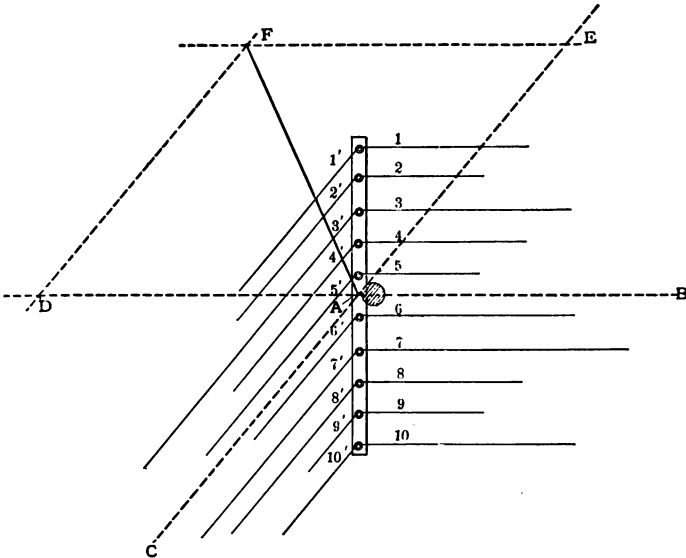
FIG. 18.—PLAN OF CORNER IN POLE LINE.
