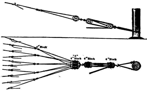
FIG. 114.—PULLING-UP WIRE.
