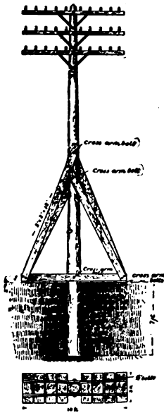
FIG. 85.— PLATFORM FOUNDATION.
