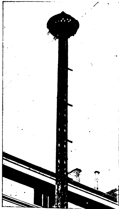
FIG. 36.— LATTICED DISTRIBUTING POLE.
