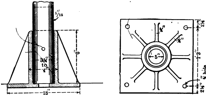
FIG. 140 — POLE BASE FOR WOOD ROOFS.
