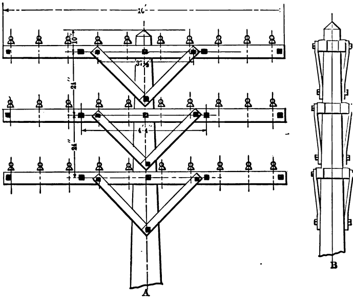
FIG. 92 A AND B.—DOUBLE ARMING.
