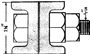
FIG. 139.— SECTION OF CROSS ARM.
