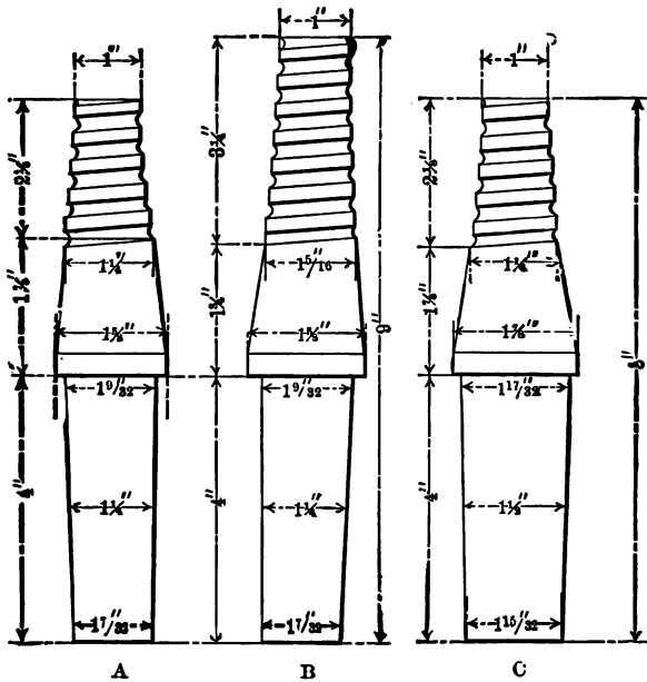
FIG. 58.—WOODEN PINS.
