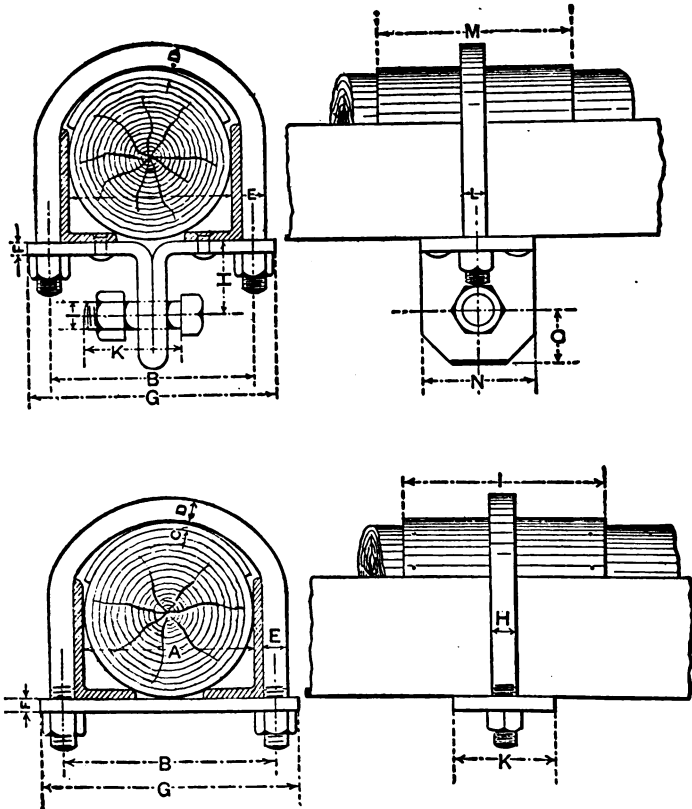
FIG. 26.—CROSS SECTIONS AND SIDE ELEVATIONS OF BANDS.
