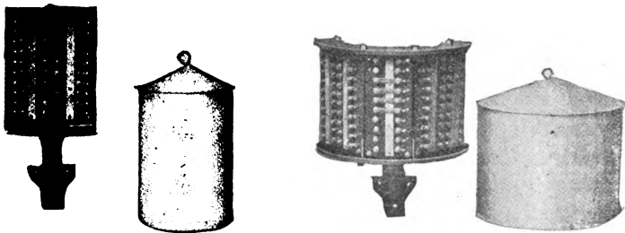
FIG. 38.—DETAILS OF POLE TOP FOR CABLE DISTRIBUTION.
