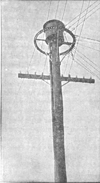
FIG. 30.— DISTRIBUTING POLE TOP, OPEN WIRE, AND CABLE.
