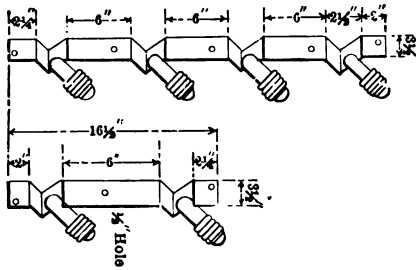
FIG. 52.— IRON BRACKETS.
