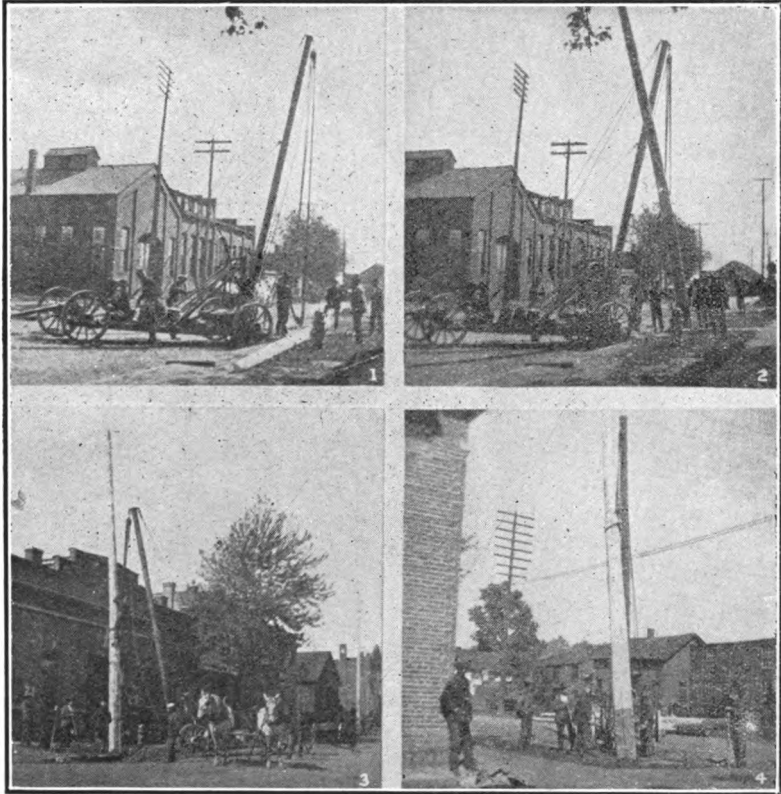
FIG. 80.—EXAMPLES OF USE OF POLE DERRICK.
