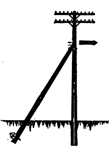
FIG. 103.— SINGLE BRACE.
