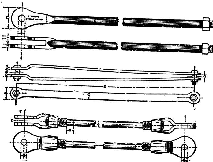
FIG. 27.—DETAILS OF GUY RODS.
