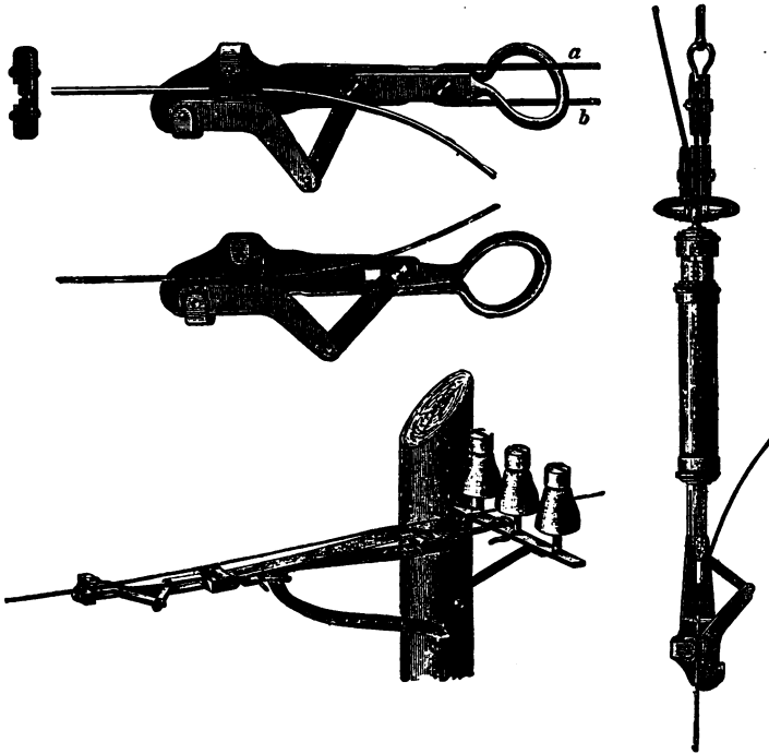
FIG. 115.—LINE DYNAMOMETER.
