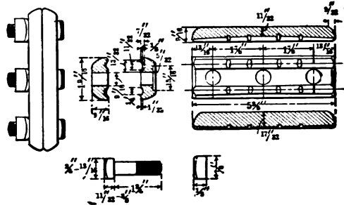
FIG. 77.— STRAND CLAMP DETAILS.
