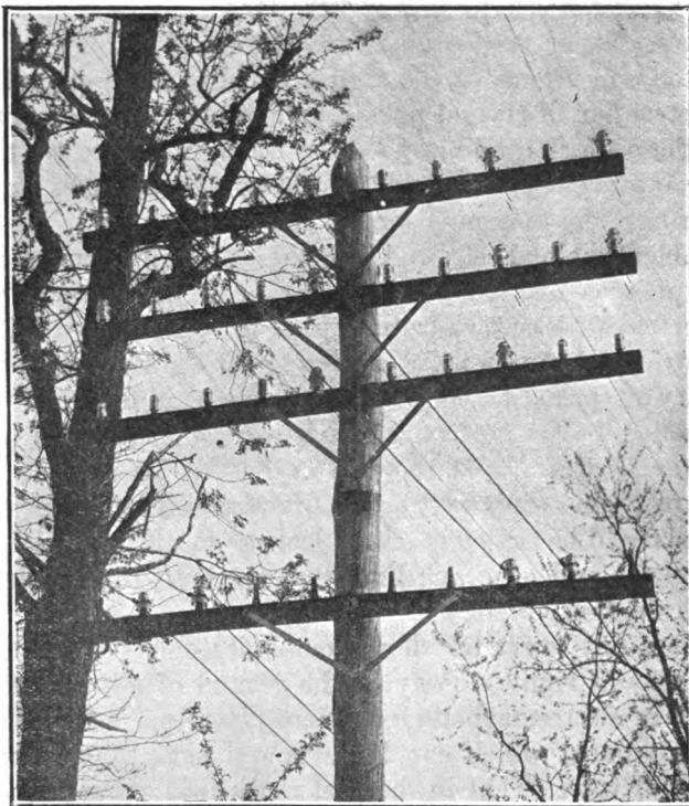
FIG. 11.—POLE CARRYING ELECTRIC LIGHT AND TELEPHONE WIRES.
