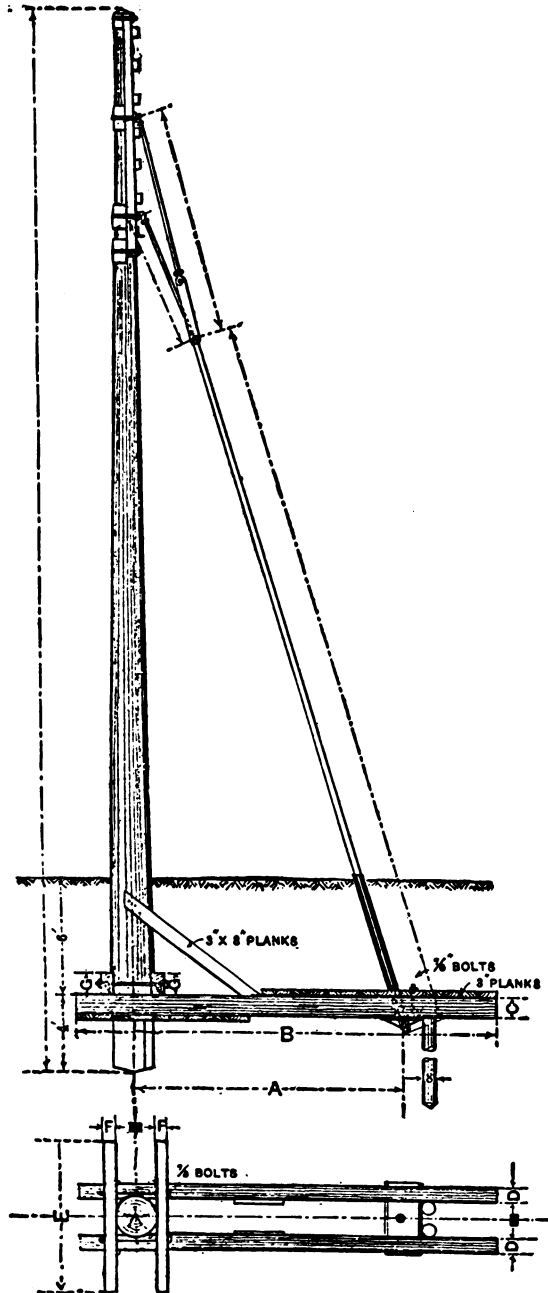
FIG. 24.—ELEVATION AND PLAN OF COMPOSITE ANCHOR POLE.
