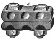
FIG. 75.— TWO-BOLT CLAMPS.
