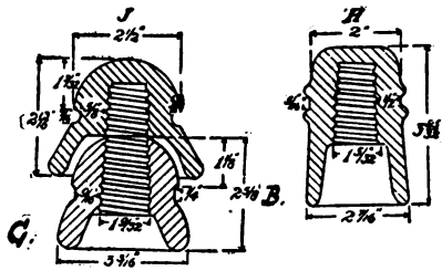
FIG. 61. B AND G.—INSULATORS.
