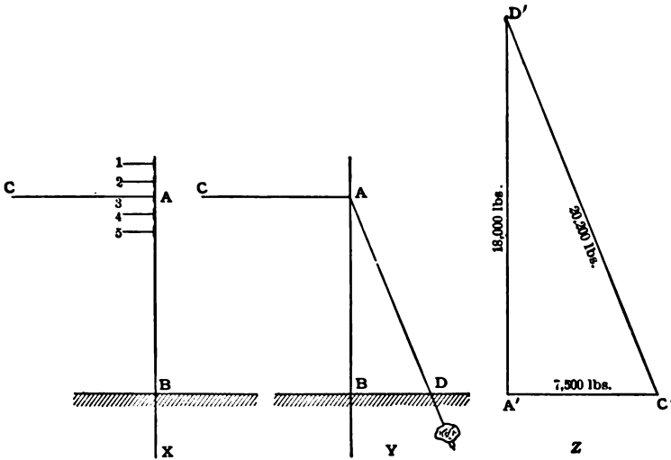
FIG. 19.—GUY DIAGRAM.
