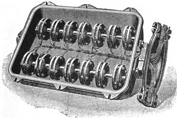
FIG. 4.—CABLE COMPENSATING COILS.
