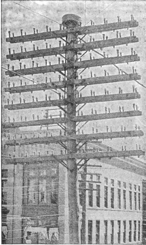
FIG. 32.— DISTRIBUTING POLE, STERLING HEAD.
