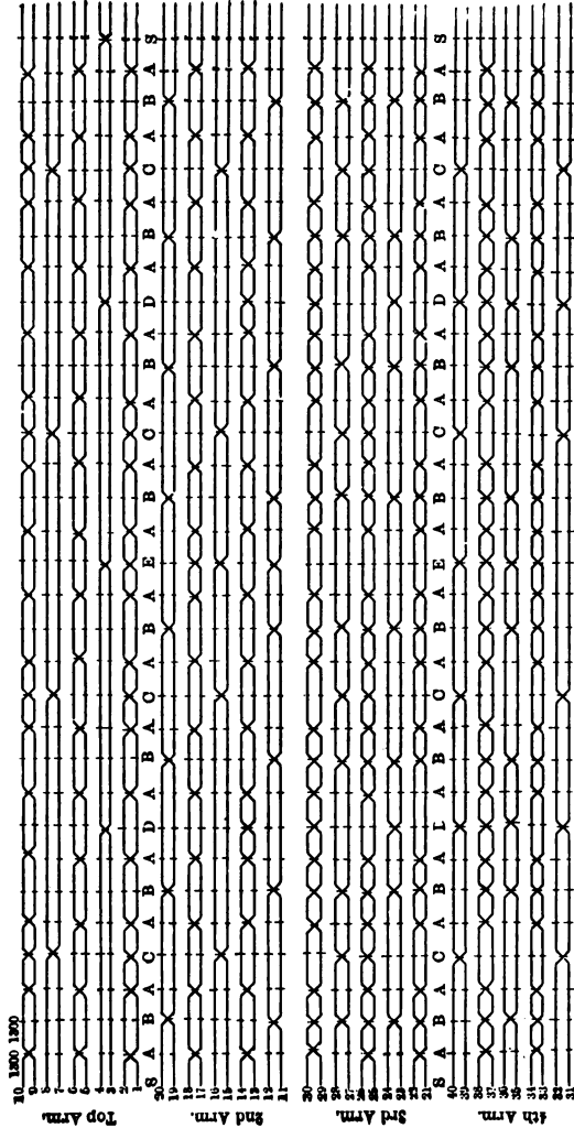
FIG. 126.—TRANSPOSITIONS FOR TWENTY-WIRE LINE.
