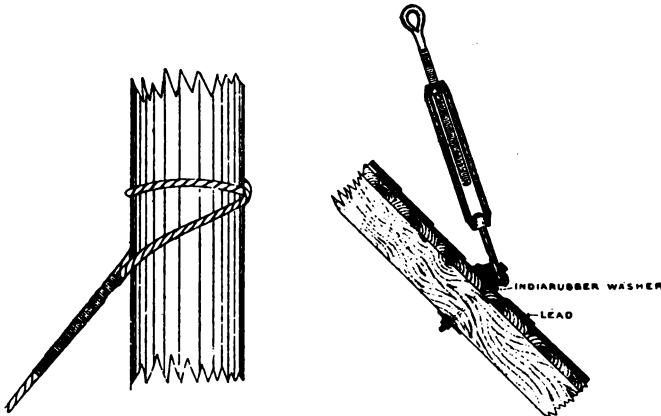
FIG. 142.—GUY AT POLE.
