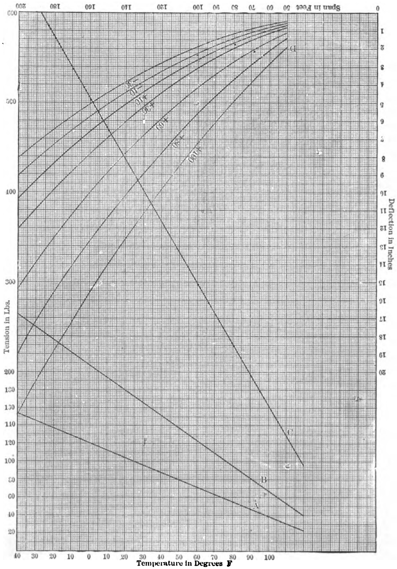
FIG. 116.—SAGS AND TENSIONS.
