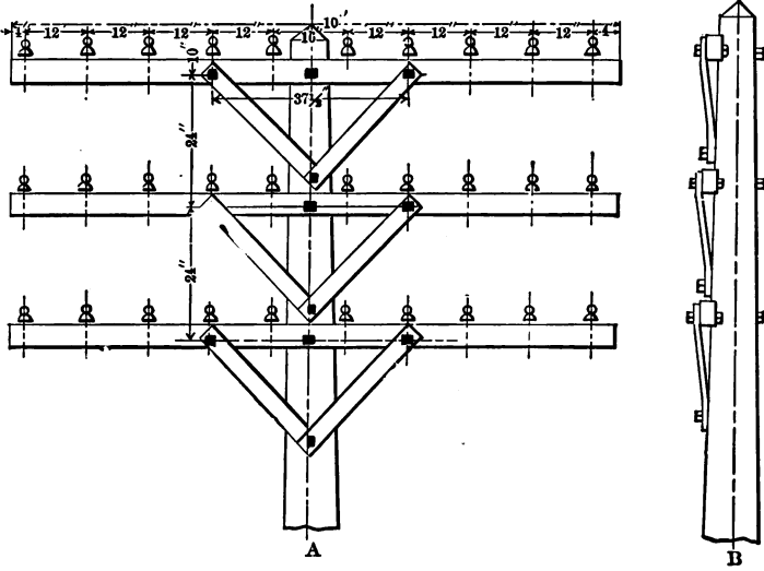
FIG. 90.— ATTACHMENT OF FRONT BRACES.
