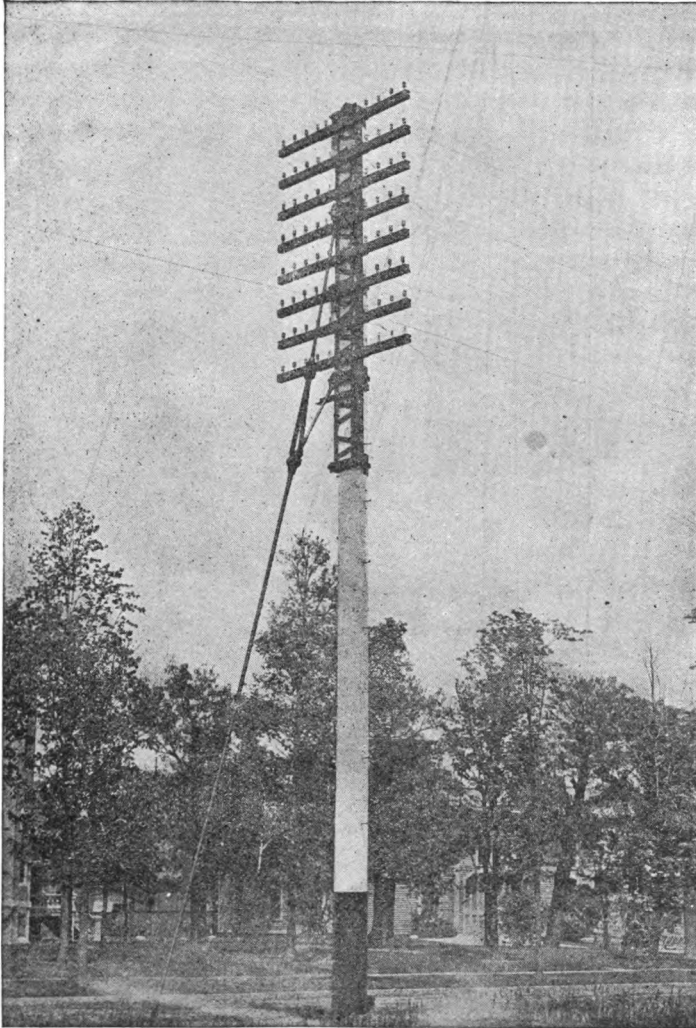
FIG. 23.— COMPOSITE ANCHOR POLE.
