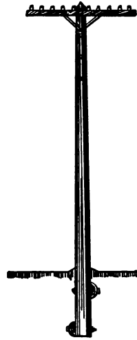
FIG. 84.— LOG FOUNDATION.
