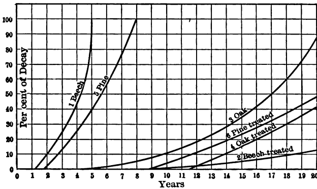
FIG. 16.—CURVES SHOWING RELATIVE LIFE OF TREATED AND UNTREATED WOODS.
