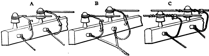
FIG. 129.—SUBSCRIBER DROP WIRES.
