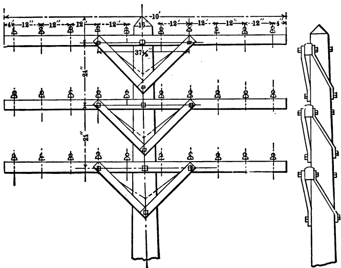
FIG. 91.— ATTACHMENT OF REAR BRACES.
