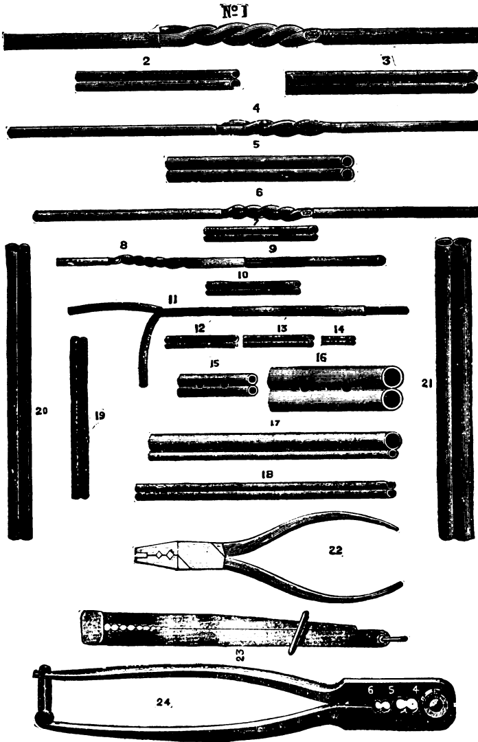
FIG. 120.—M'INTIRE JOINTS. 16
