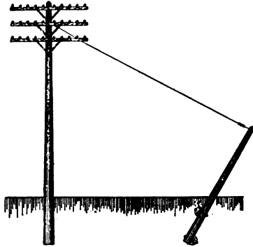
FIG. 97.—UNANCHORED GUY STUB.
