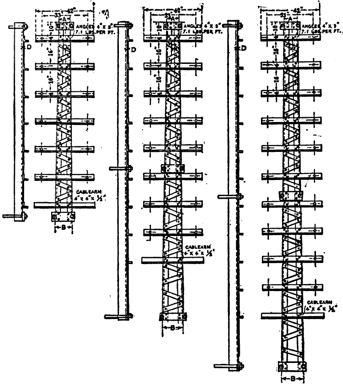
FIG. 25.—DETAILS OF LATTICE FOR COMPOSITE POLE TOP.
