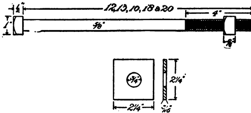
FIG. 65.— CROSS-ARM BOLTS.
