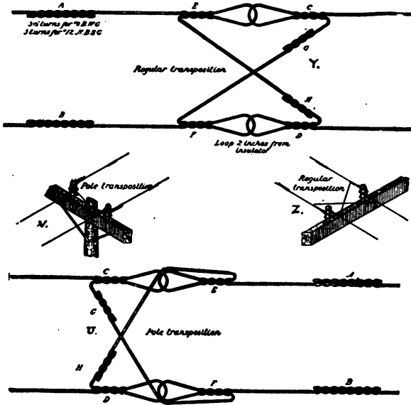
FIG. 127.—DETAILS OF TRANSPOSITION.
