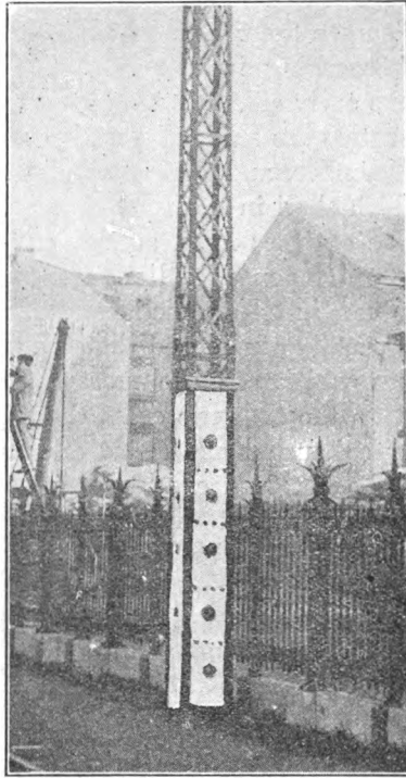
FIG. 14.—BELGIAN POLE CONSTRUCTION AT BASE.
