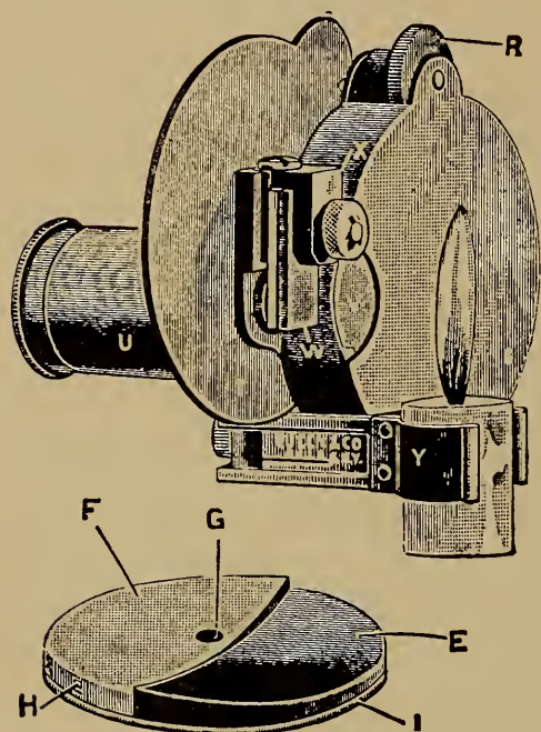
FIG. 8. Dare's hemoglobinometer.
