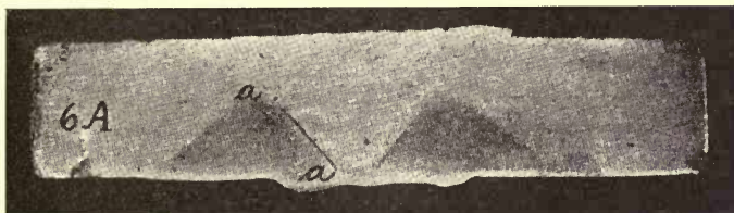
FIG. 76.— Unwelded place in seam (a-a) in consequence of improper holding of the burner.
