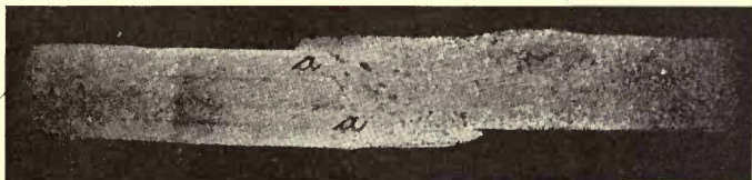
FIG. 72.— Evidence of superheating of a welding seam and unwelded spots (a. a.).
