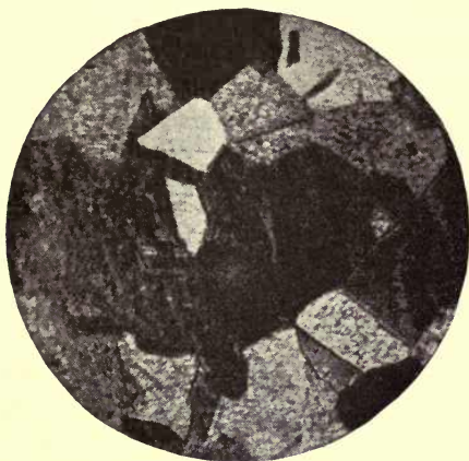
FIG. 48. — Micro-photograph of nickel steel bar — unmagnetic. (Magnified 300 diameters)
