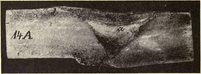
FIG. 74.— Imperfect, superheated, and carbonized welding seam.
