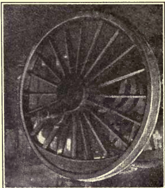
FIG. 58.— Locomotive drive wheel with cracks in spokes repaired by autogenous welding.
