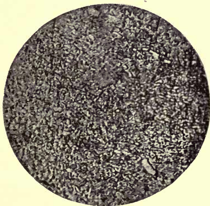
FIG. 49.— Micro-photograph of high-speed steel bar. (Magnified 80 diameters)
