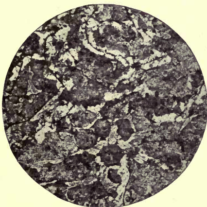
FIG. 51. — Micro-photograph of white iron. (Magnified 300 diameters)
