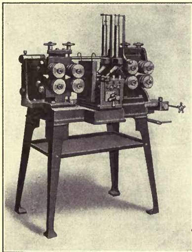
FIG. 124.— Pipe welding machine equipped with mechanically operated rolls.
