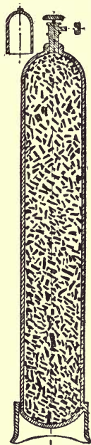
FIG. 16.— Cross section of acetylene dissolved bottle.
