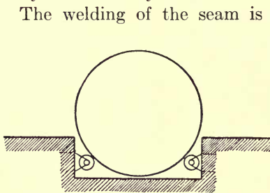
FIG. 90.—Diagram of pit equipped with rolls for welding circumferential seams.
