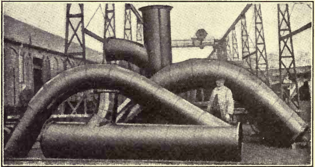
FIG. 120. — Large pipe elbows made from several sheet segments by autogenous welding.
