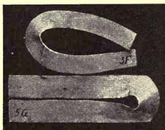
FIG. 53. — Good welds after having been subjected to severe bending test.
