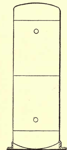
FIG. 101. — Support ring applied to a vertical cylindrical vessel.
