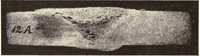
FIG. 70. — Evidence of superheating of a welding seam.
