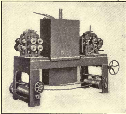
FIG. 125. — Pipe welding machine equipped with oil preheater.
