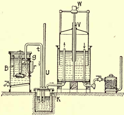
FIG. 11. — Stationary “carbide to water” acetylene generator where carbide is introduced in a closed drum —
