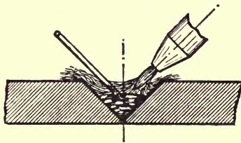
FIG. 57.— Method of stirring the molten metal with the filling bar during the welding operation to destroy the films of oxide.
