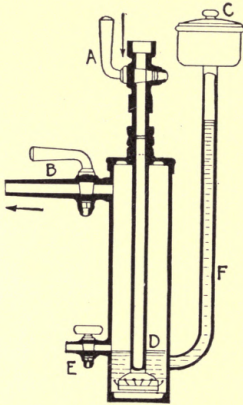
FIG. 27. — Cross section of water seal — Fouché system.
