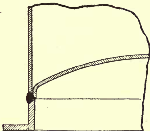
FIG. 100.— Angle-ring welded on the bottom of a cylindrical vessel.
