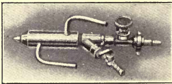
FIG. 127.—Welding burner equipped with water cooling device for pipe welding machine.
