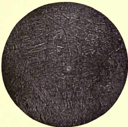
FIG. 47. — Micro-photograph of steel bar containing about 0.75% carbon — hardened. (Magnified 80 diameters)
