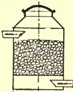
FIG. 17.— Chemical purifier using hygroscopic cleansing mass.
