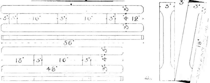
PLANS AND ELEVATIONS OF TOP FRAMES
