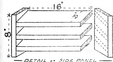
DETAIL OF SIDE PANEL
