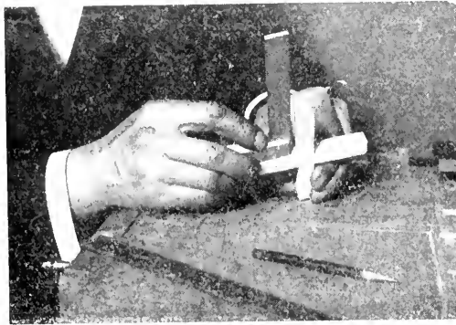
FIG. 25. TESTING ANGLE WITH TRY SQUARE.
