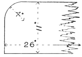
DETAIL OF SEAT-BACK
