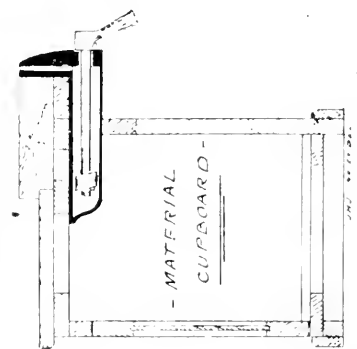
SECTION XX
