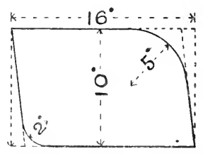
DETAIL OF SEAT-ENDS
