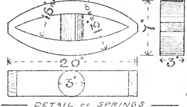
DETAIL OF SPRINGS
