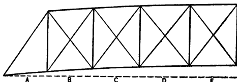
Diagram in Which the Panels at A is Shortest, and at E Longest. The Bolts Radiate to the Center of the Arch.
