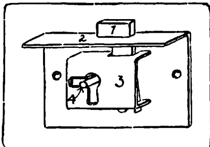
Fig. 236. Rim-lock, for Drawer. 1. Bolt. 2. Selvage. 3. Box. 4. Key-pin.
