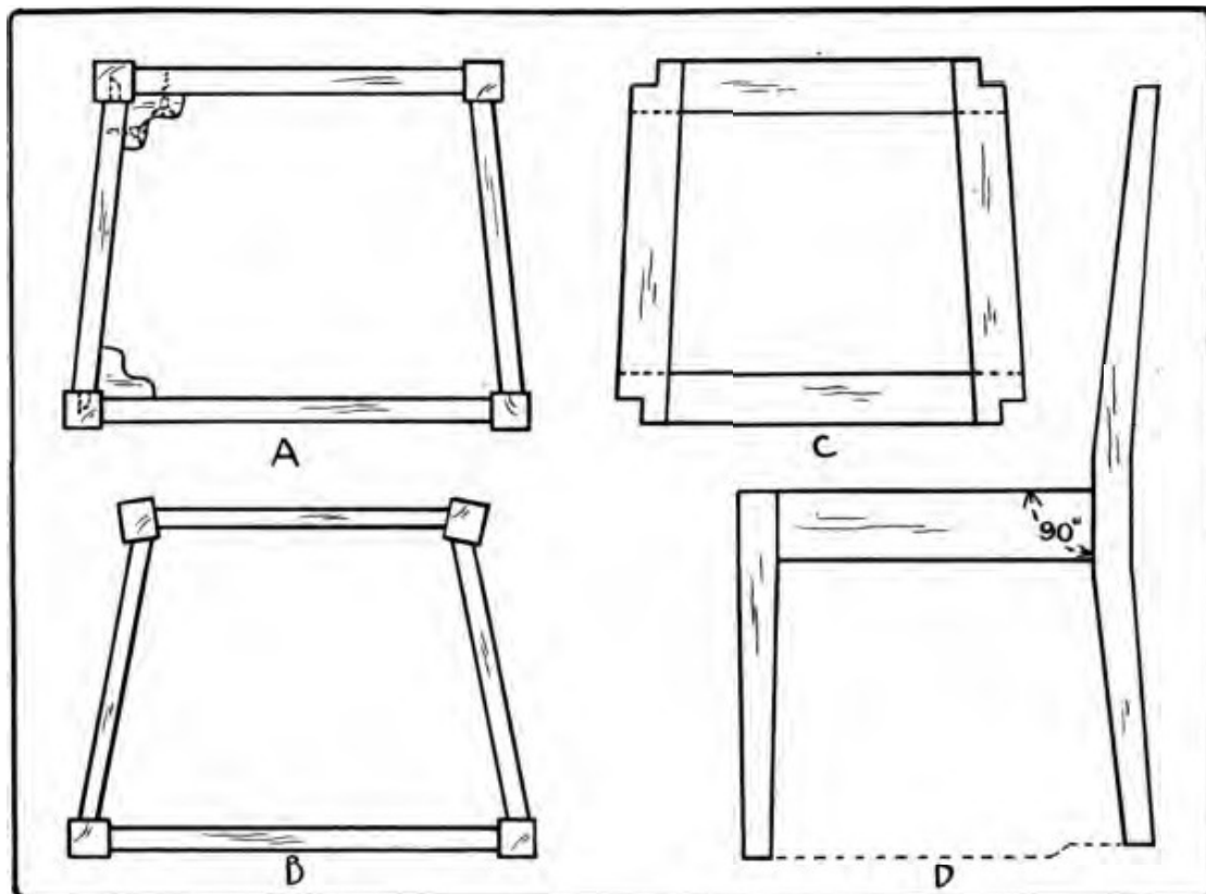
Fig. 298. Chair Construction.
