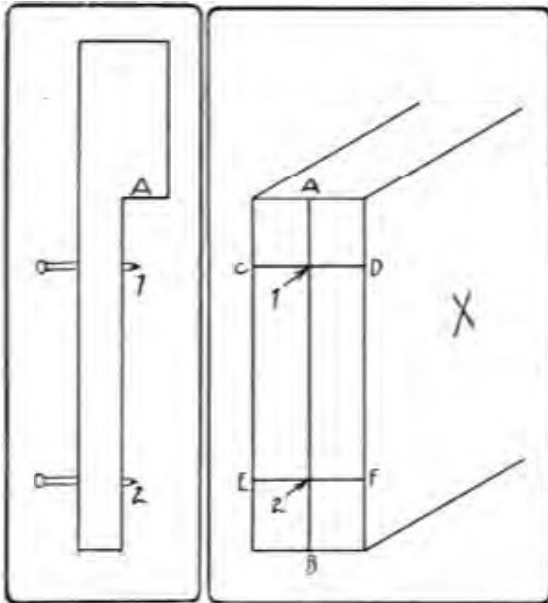
Fig. 249. Laying out a Dowel Joint.
