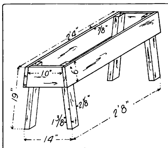
Fig. 171. Saw-Horse.
