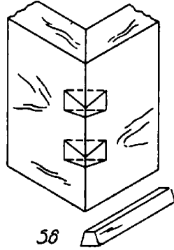
Slip-dovetail miter
