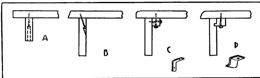
Fig. 297. Methods of Attaching Table Top to Rails.
