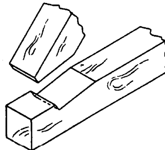
64 Oblique thrust
