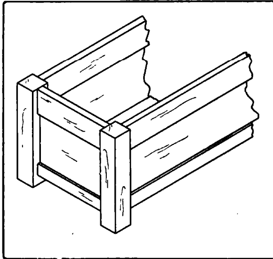
Fig. 290. Chest Construction.
