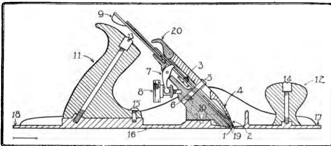
Fig. 101. Section of Jack-Plane.
