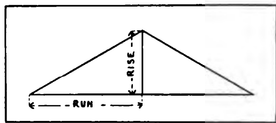
Fig. 198. The "Run" and "Rise" of a Rafter.
