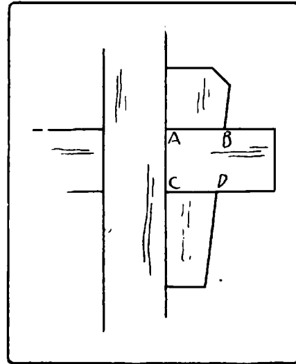
Fig. 252. Keyed Mortise-and-Tenon Joint.
