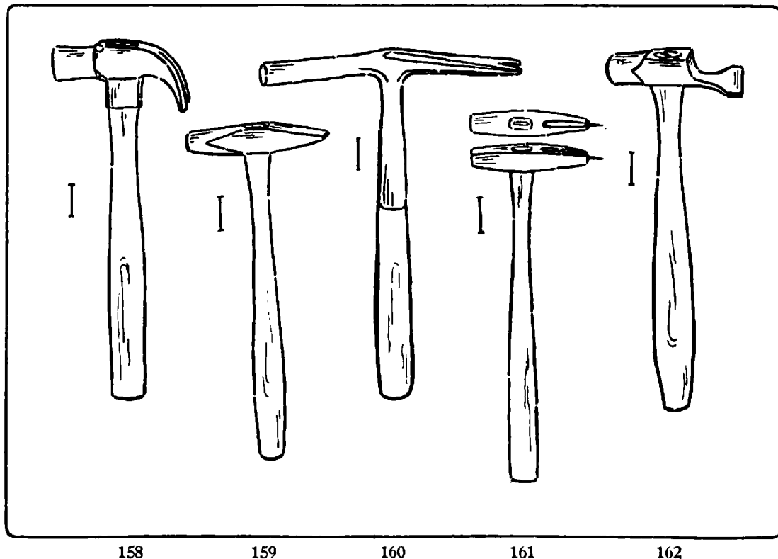
Fig. 158. Claw-Hammer,
