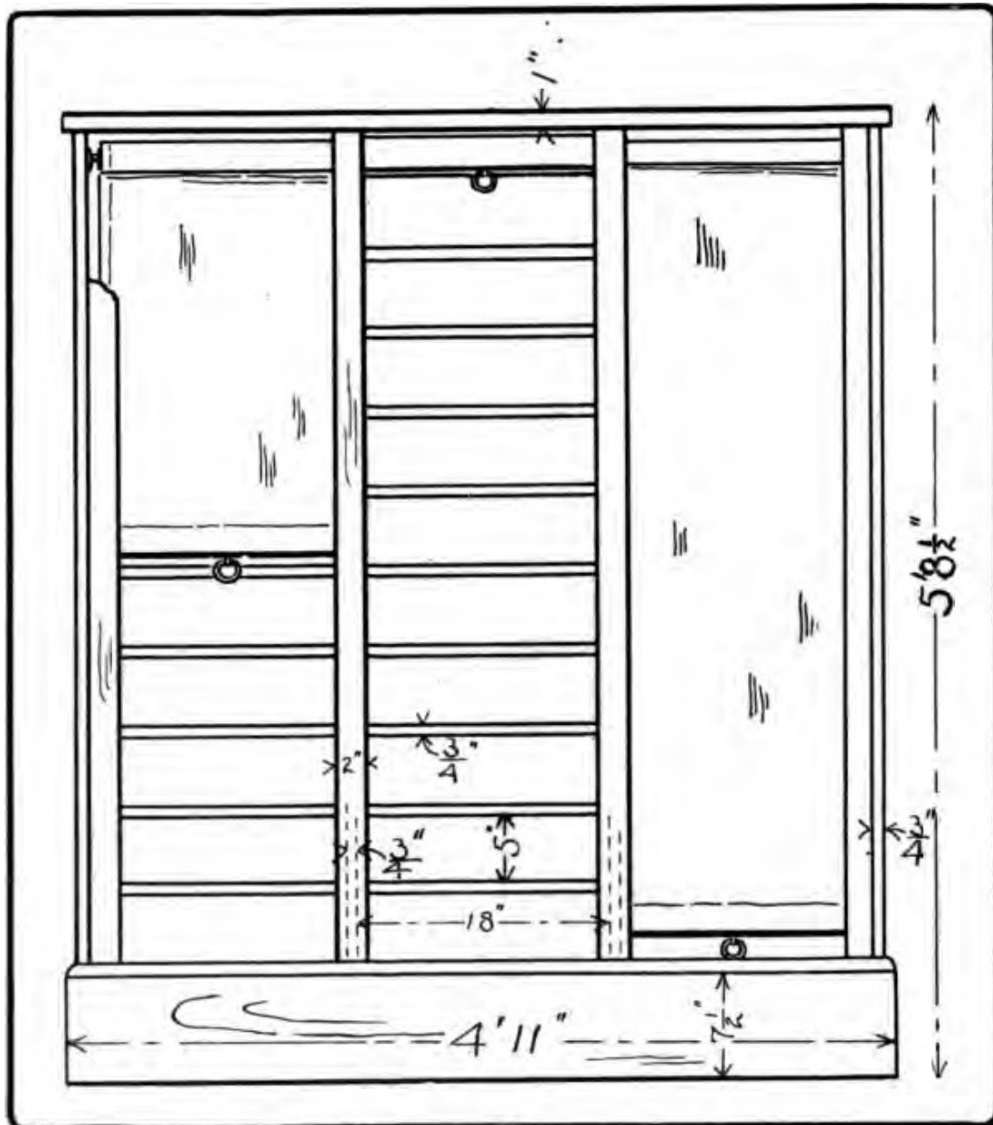
Fig. 241. An Inexpensive Locker for Unfinished Work.
