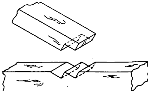
63 Square thrust
