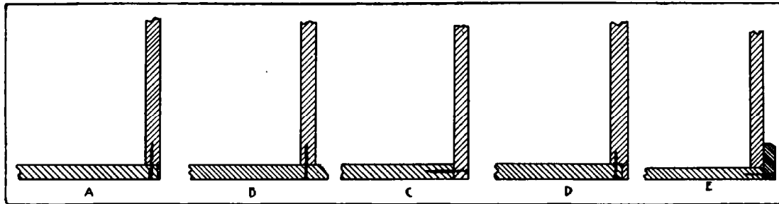
Fig. 284. Methods of Attaching Box Bottoms.
