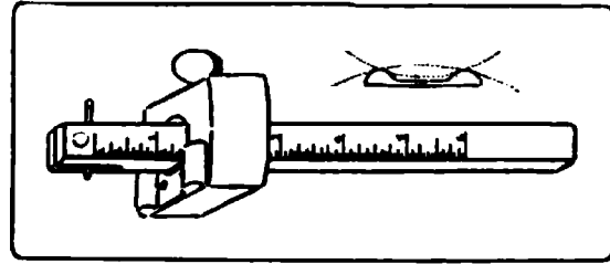
Fig. 215. Marking-Gage for Curves.
