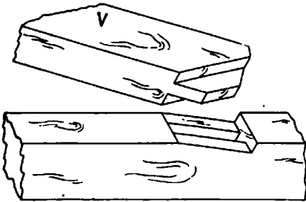
67 Oblique mortise-and-tenon
