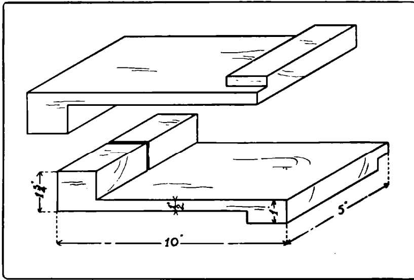
Fig. 179. Bench-Hook.
