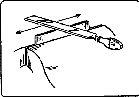
Fig. 153. Sharpening a Cabinet-Scraper: 1st Step, Drawfiling.
