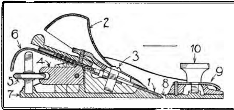
Fig. 103. Section of Block-Plane.
