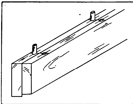
Fig. 262. Edge-to-Edge Joint, Doweled.
