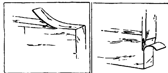
Fig. 61 Edge and Wedge Action With the Grain.
