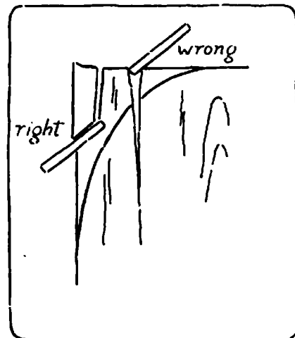
Fig. 75. Right and Wrong Ways of Perpendicular Chiseling.
