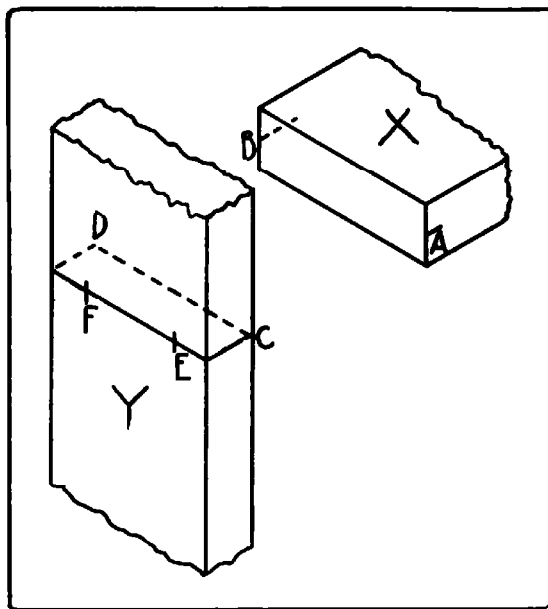
Fig. 246. Lay-out for Thru Doweling.
