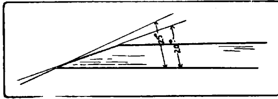
Fig. 78. Grinding Angle, 20°; Whetting Angle, 25°.
