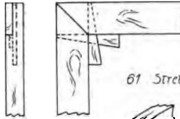
Double dovetail keyed
