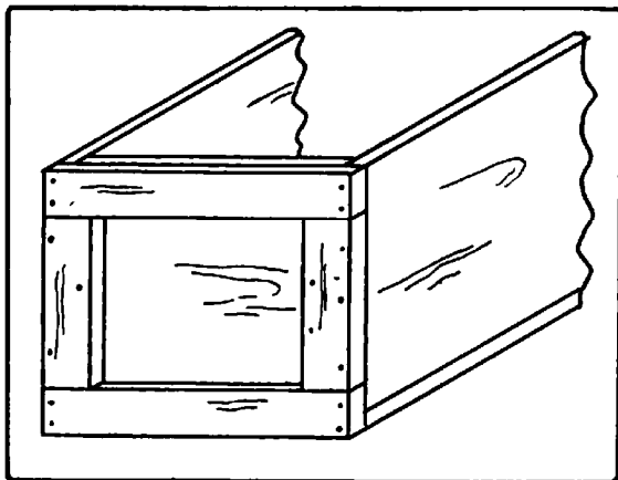
Fig. 283. Reinforced Butt Joint in Box.
