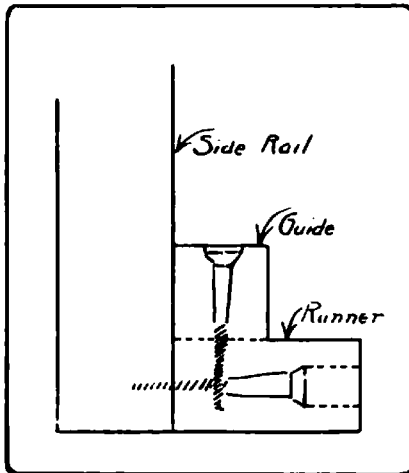
Fig. 295. Drawer Mechanism.
