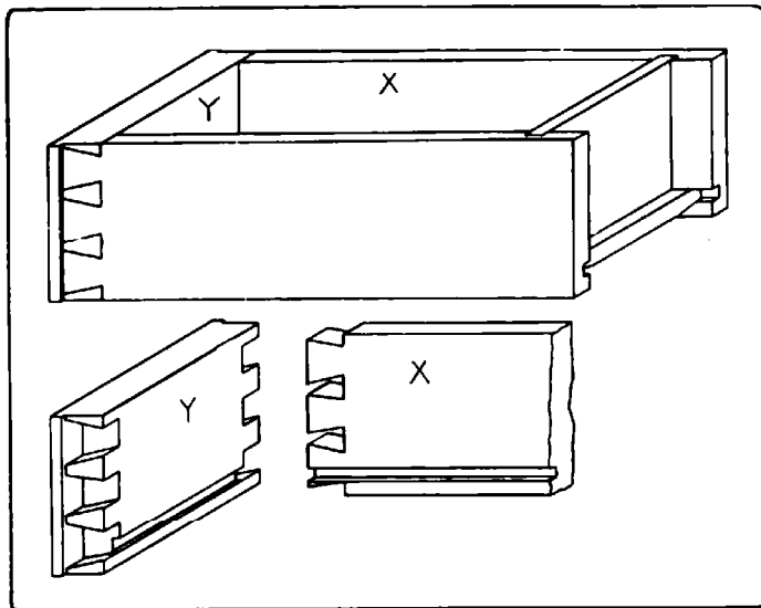
Fig. 287. Dovetailed Drawer Construction.
