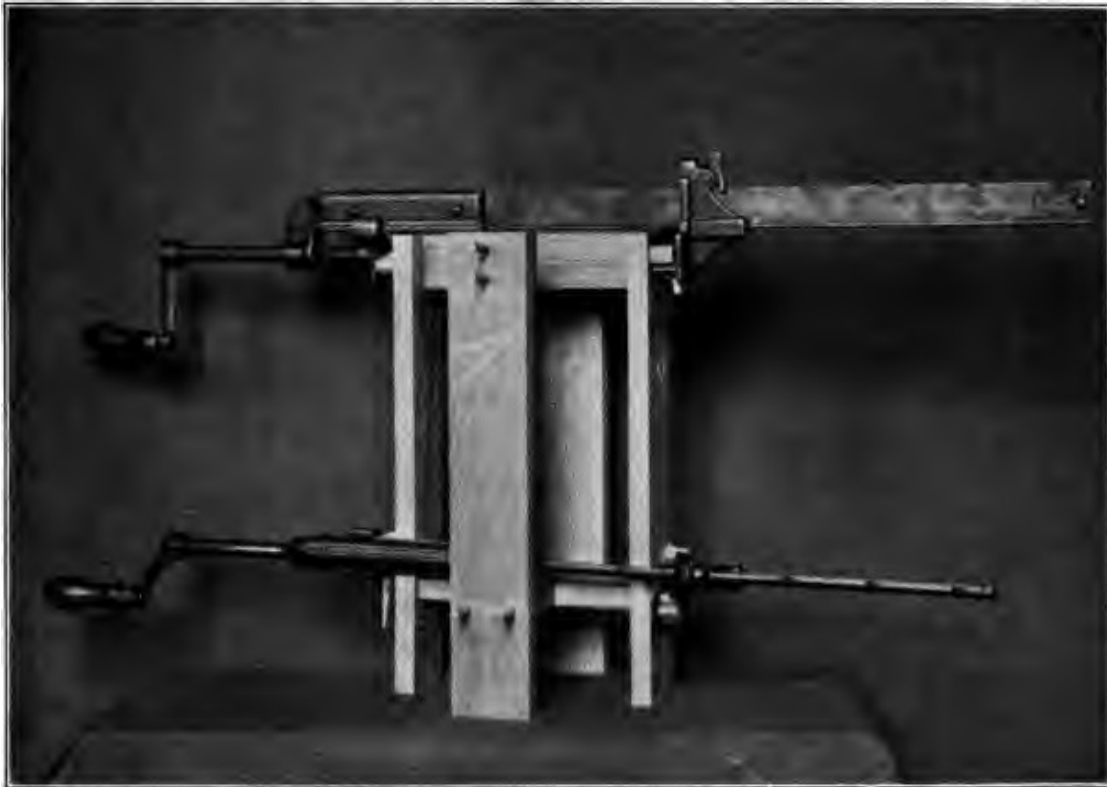
Fig. 248. Gluing Up a Four-legged Stand.
