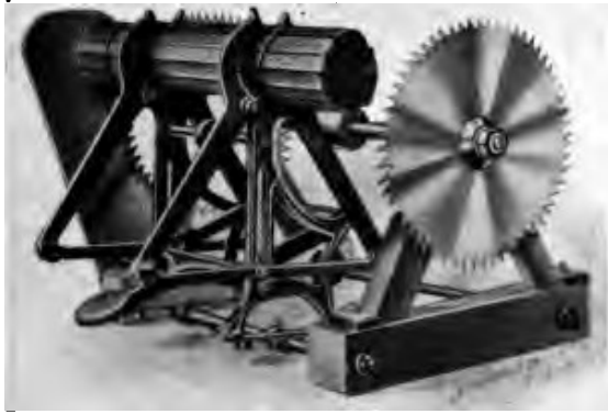
Fig. 51. Combination Lath-Binder and Trimmer. With this machine the operator can trim the bundles of lath, simply by tilting the packing frame over from him causing the bundles to pass between the saws, thereby trimming both ends at one movement.
