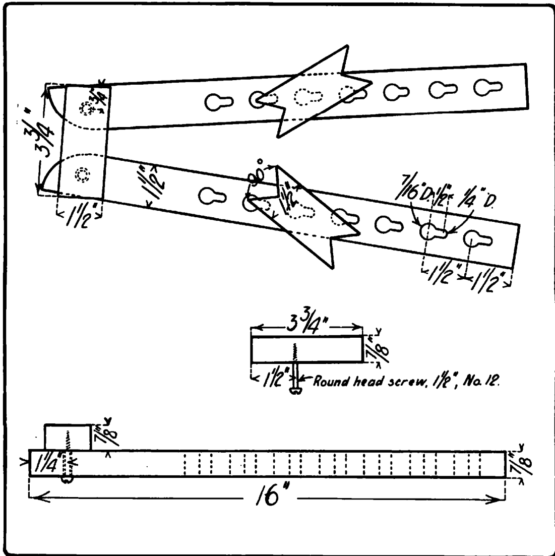
Fig. 255. Picture-Frame-Clamp. (See also Fig. 254.)
