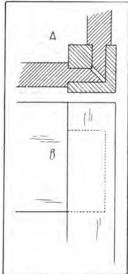
Fig. 291. A. Cross-Section Thru Back Left Leg and Adjoining Rails of Table. (Plan). B. Elevation, Showing Wide Shoulder on Tenon of Rail.
