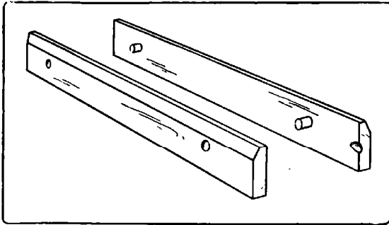
Fig. 205. Winding-Sticks, 12 inches Long.
