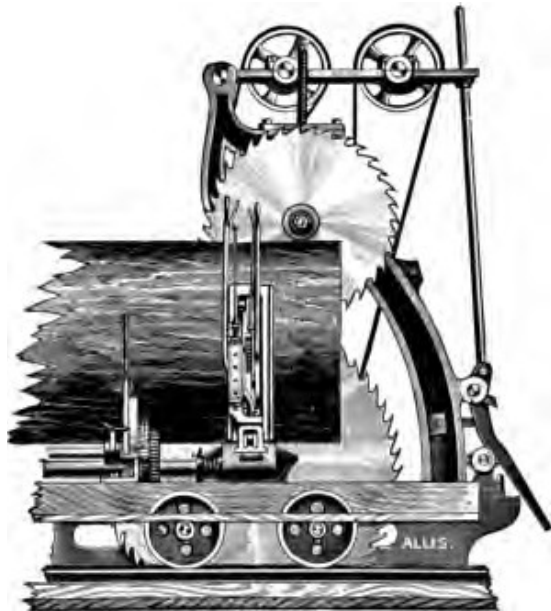
Fig. 32. Double Circular-Saw and Carriage.
