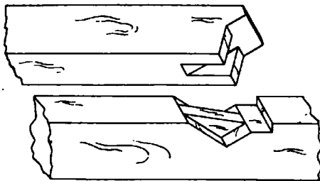
68 Bridle
