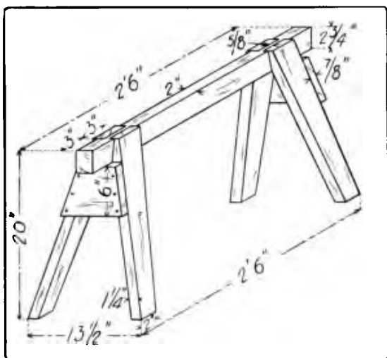
Fig. 170. Saw-Horse.
