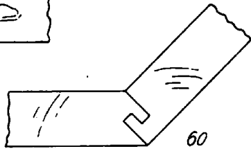
Double-tongue miter
