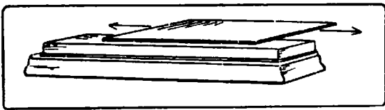
Fig. 154. Sharpening a Cabinet-Scraper: 2nd Step, Whetting.
