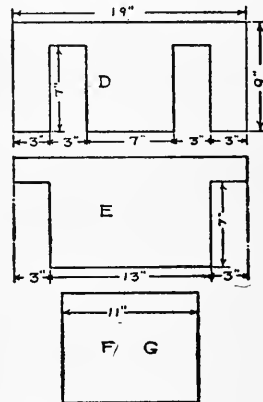
FIG. 69. PARTITIONS FOR SECOND FLOOR.
