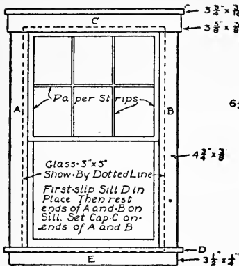
FIG 85 WINDOW TRIM FIRST AND SECOND STORY
