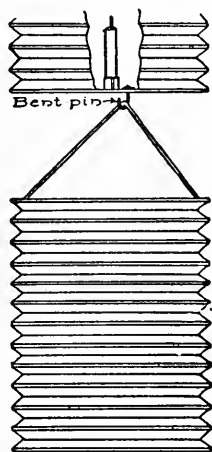
FIG. 296. Schemes for Attaching Lanterns to Kite-strings.
