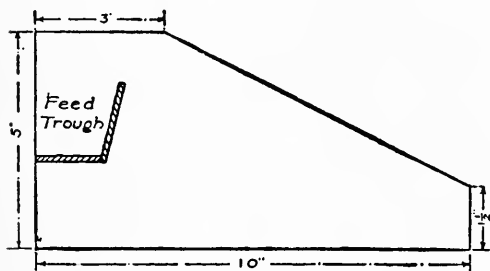
FIG. 117. — Stall Partitions.
