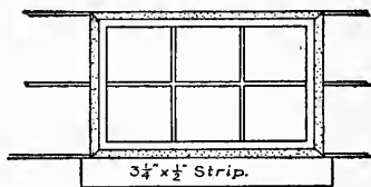
FIG 83 BASEMENT WINDOWS
