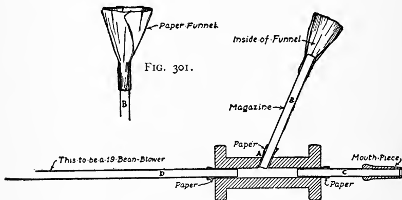
FIG. 300. — A Section through the Bean-blower. A Magazine Bean-blower.
