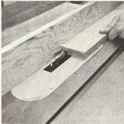
Cutting the Groove in the Stile
