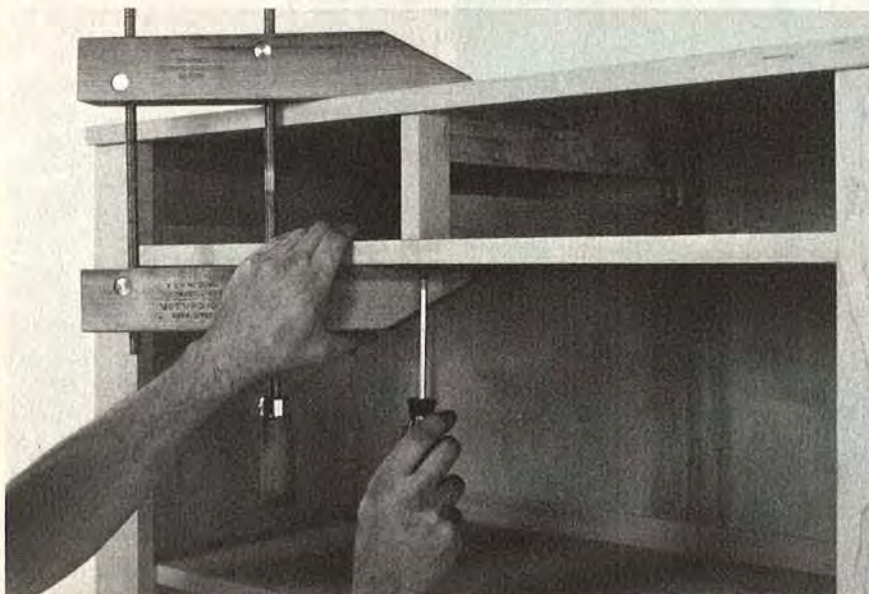
Screwing the Top Shelf to the Drawer Divider
