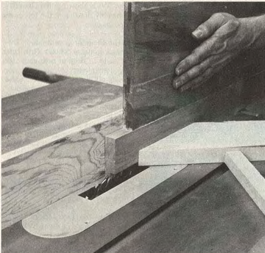
Cutting the Rabbet in Panel Edge
