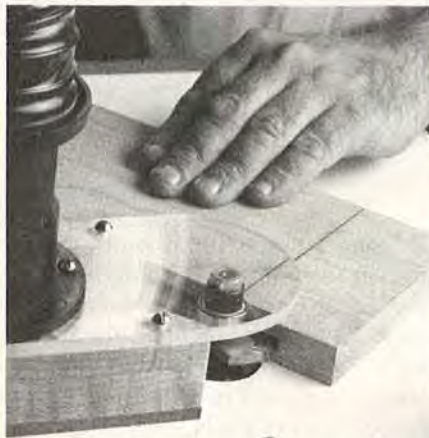
Cutting Stopped Groove for Spline
