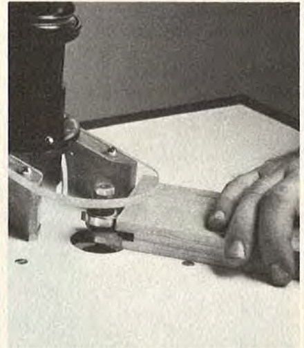
Cutting the End-Spline Groove
