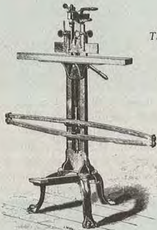
IMPROVED FOOT-POWERED MORTISING MACHINE
