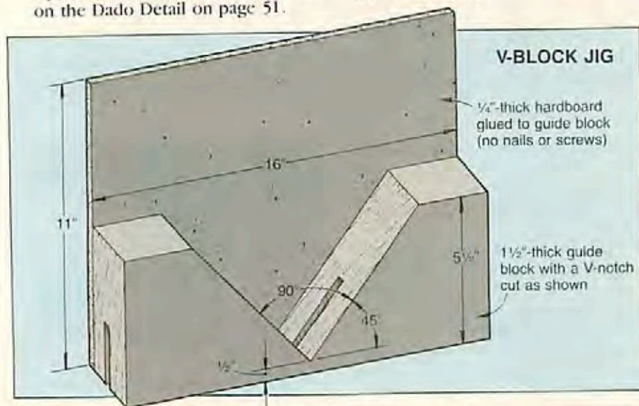
Use a V-block jig to cut the spline slot in each frame corner.
