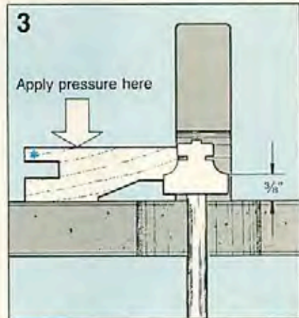
3 Switch to a \frac{3}{16} " round-over bit with pilot. While cutting, push down on back side of stock to keep it from rocking.
