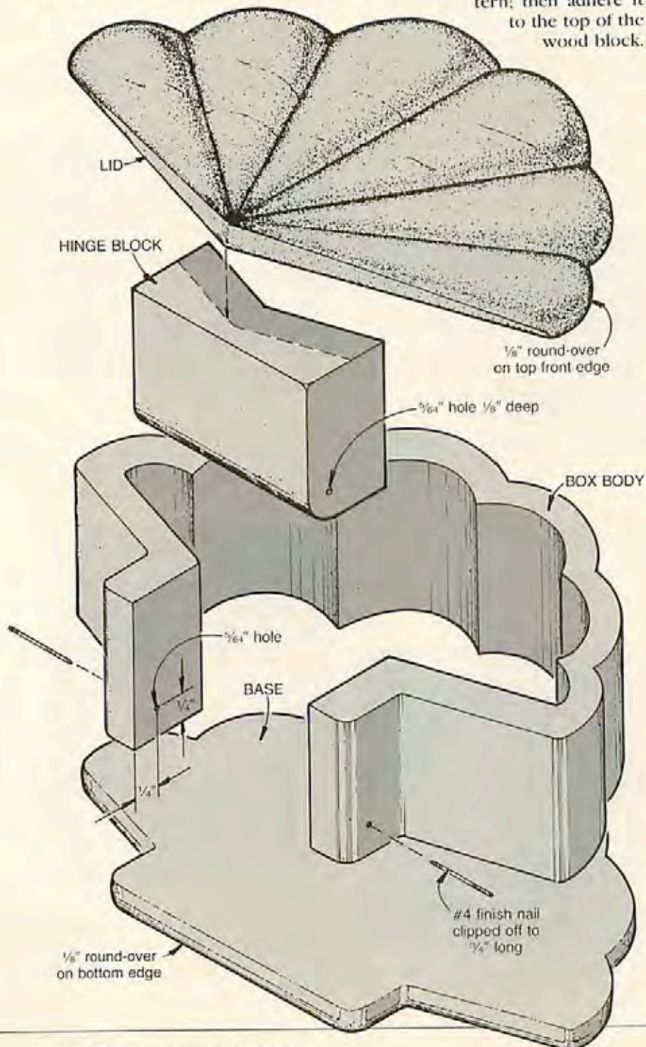
Cut slightly outside the marked perimeter line to cut box to shape.
