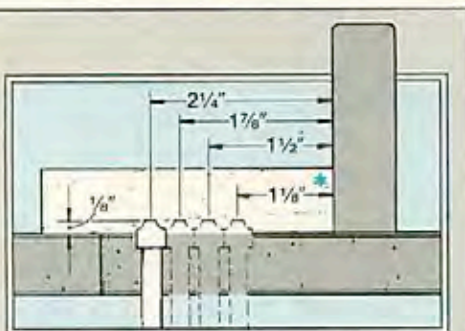
Start with \frac{3}{4} \times 3\frac{1}{2} " stock. Use a \frac{3}{8} " beading bit to make cuts where shown by moving the fence.
