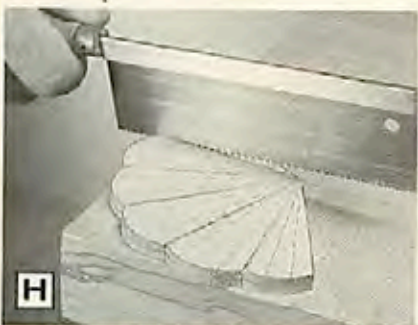
Cut angled kerfs with a fine-toothed saw at the marked lines.
