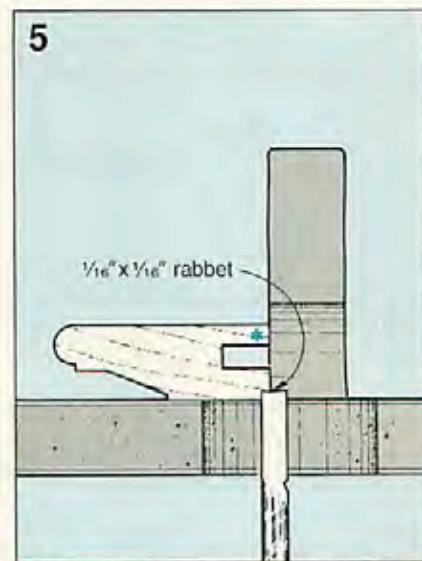
5 Switch to a \frac{1}{16} " straight bit. Set bit height and fence position to cut a \frac{1}{16} " \times \frac{1}{16} " rabbet. Flop piece as shown.
