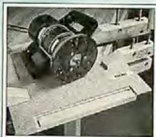
Template with a routed groove in an end frame.
