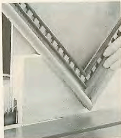
Use a V-block jig to cut the spline slot in each frame corner.
