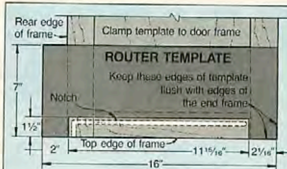
Template with a routed groove in an end frame.
