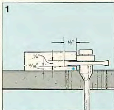
1 Start with \frac{3}{4} \times 2\frac{1}{8} " stock. Use a \frac{1}{4} " slot-cutter bit to rout a groove along one edge of the piece, where shown on the drawing.
