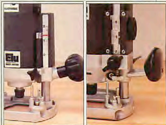
Depth adjustments on most units work like the one on the small Elu, left . The large Elu ( right ) has a more sophisticated mechanism.
