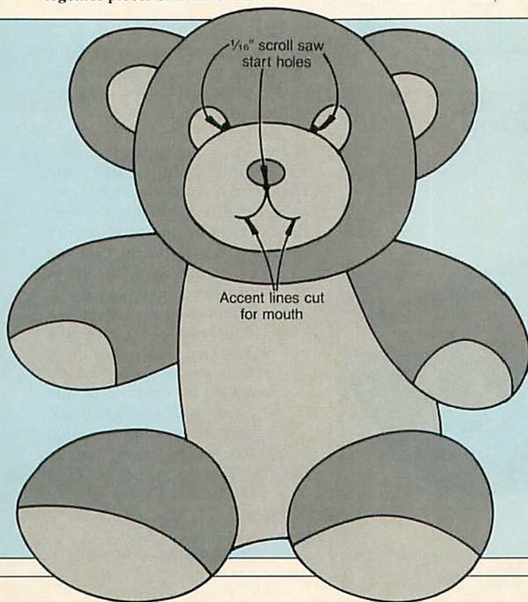
Cut the parts to shape from the taped-together pieces of walnut and oak.
