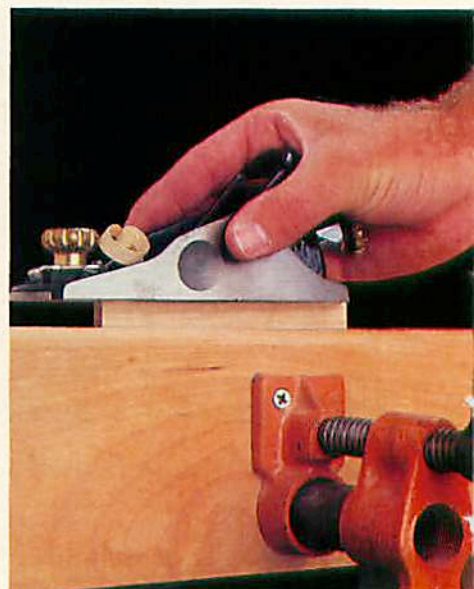
If you've glued down a too-wide strip as shown at left, pop it off with a chisel. Then, plane a new strip to fit (right).
