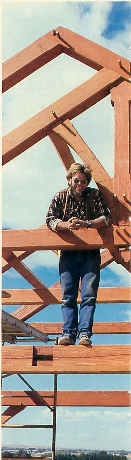
Sam assembles a king-post strut on the end section of the timber frame.
