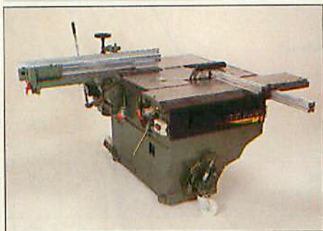
Above: Tilting-arbor shaper is a Felder exclusive; rip fence for table saw slides to far side of jointer table, providing a 39" rip capacity. Right: Felder BF5/41: Largest and most expensive machines.
