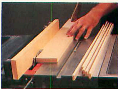
On the table saw, position the fence \frac{1}{4} " from the blade, and rip stock into \frac{1}{4} "-thick strips, using a push stick for safety.
