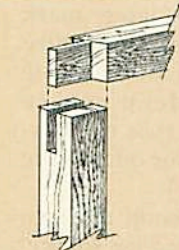
Open mortise and tenon
