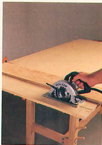
Clamp a straightedge to the workpiece, and cut the top to finished size.
