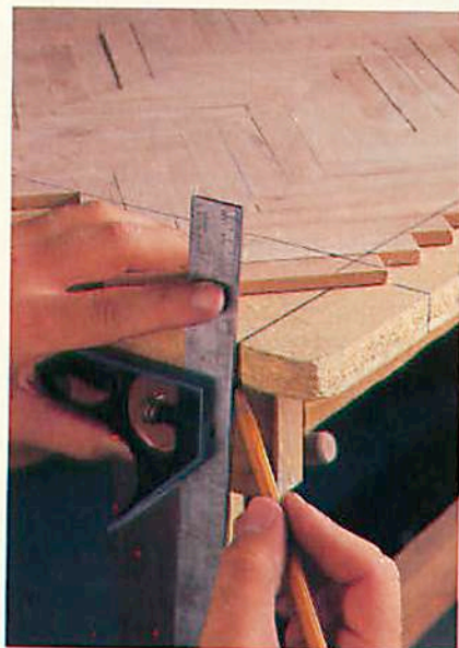
Mark the panel's finished size, then transfer the marks to the back side.
