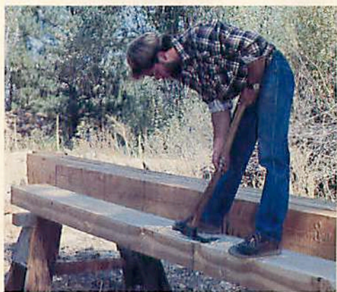
Above: With an adze, Sam smooths one of the pine timbers for his picnic-table gazebo. He pulls the adze toward him.
