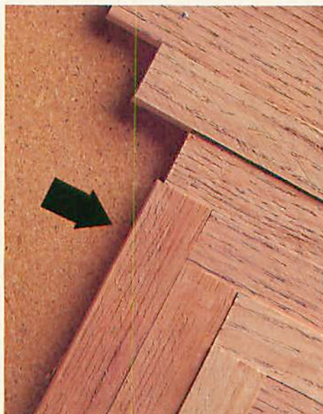
If you've glued down a too-wide strip as shown at left, pop it off with a chisel. Then, plane a new strip to fit (right).
