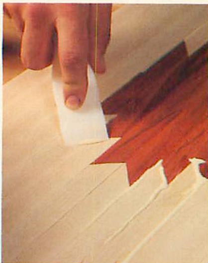
If your project consists of two or more wood species, use this method: Force glue into the cracks with a plastic putty knife ( left ). Then, run a palm sander over the glue lines to force sawdust into them ( right ).
