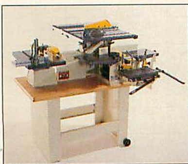
Left: Kity K5: To switch functions on this inexpensive, one-motor machine, you change the drive belt from one component to another. Right: Kity DD: You can begin with the basic drive unit and one or two machines, then add the rest as need and budget allows. Center: Central control panel on the Kity DD operates electric clutch (at bottom of photo) to switch functions.
