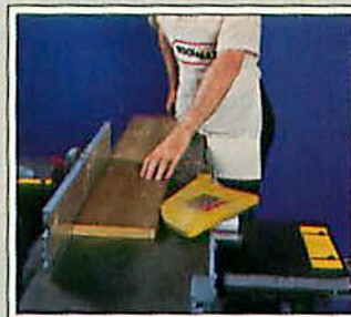
1 With the tool in the jointer mode, Ray Owen joints one side and one edge of the oak stock.
