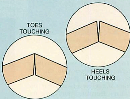
Dry-clip the test staves to check for angle accuracy.
