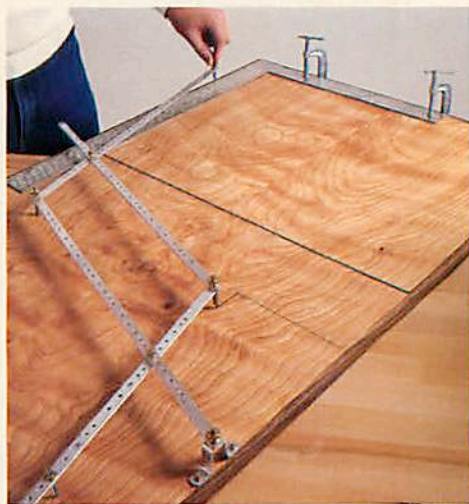
Follow the outline of the copy-area rectangle with the tracing point to mark the 4:1 ratio rectangle on the drawing board. Darken lines with a felt-tip marker.
