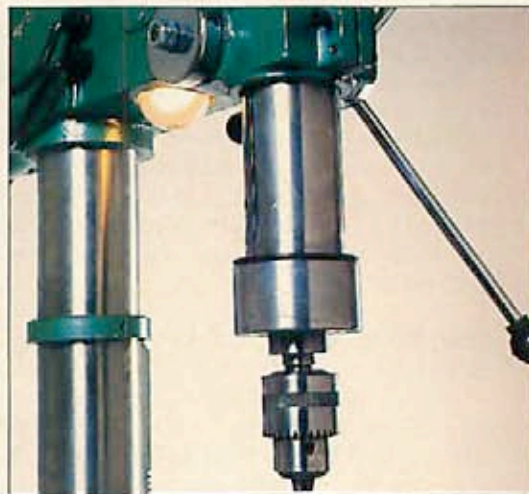
The 5¼" quill travel on the Grizzly G-1201 outdistanced all the others we tested. By adjusting the allen bolt, top center , the operator can eliminate spindle play between the quill and the head.
