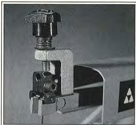
▲ When using a clamp-type holder such as the one shown above, make sure you leave a 1/16” gap between the locking screw and clamp to prevent excessive blade breakage.
