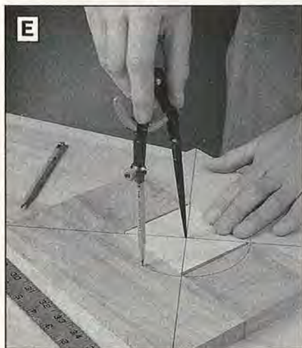
Use a scrap block and compass to draw the circular cutaway hole in the center of each layer. This makes for easier turning later.
