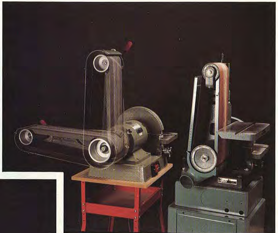
▲ We removed the belt guards for an inside look at the Grizzly model G1183 on the left, and Delta model 31-730. Our inspection revealed a more-sturdily mounted upper roller on the Delta.
