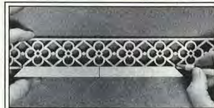
Center the filigree over the marked centerline, and mark cut lines for matching patterns at each end.
