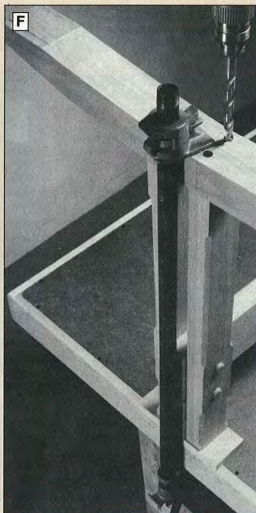
F Clamp the foot to the uprights. Mark the centerpoints, and bore the holes for the dowels.
