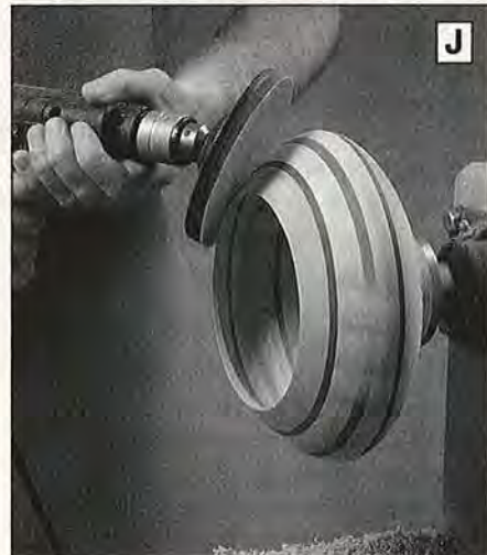
You can sand the bowl by hand, but you'll save yourself a lot of time by power-sanding. An angle drill works well on the inside wall of the bowl.
