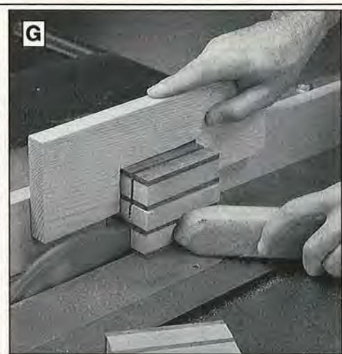
... pass the other segments through the blade. We're using a pushstick and abrasive belt cleaner to safely hold the segment.
