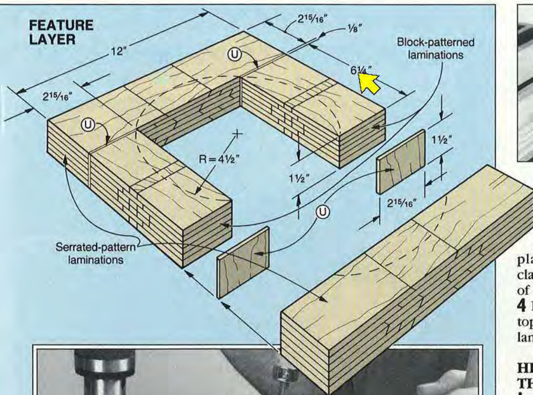
For safety, use a thin push block when cutting to length the narrow block-pattern pieces.
