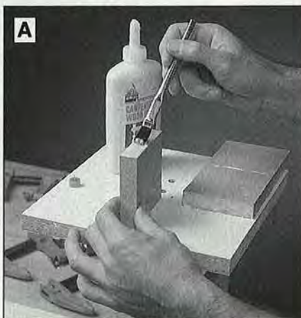
Spread liberal amounts of glue on both surfaces wherever you join two pieces. Here, we're gluing the middle segment of the bowl's bottom.
