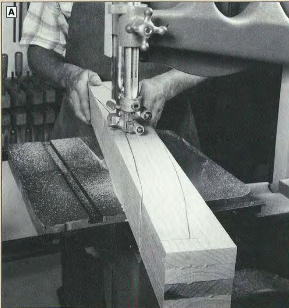
Trace the template outline onto the foot lamination, and then cut the foot to shape on the bandsaw. Later, trim the ends square on a radialsaw.
