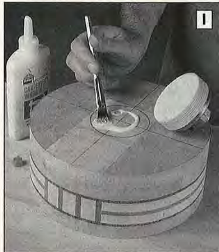
Apply glue to both the auxiliary faceplate and bowl-blank bottom. You also can use 5-minute epoxy to speed this process and spare the clamping.
